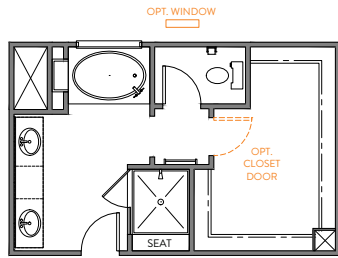
LUXURY BATH OPTION 3 42" x 60" GARDEN TUB w/CERAMIC TUB SURROUND 42" x 48" FRAMED TILE SHOWER BASE TILE WALLS w/12" TILE SEAT
