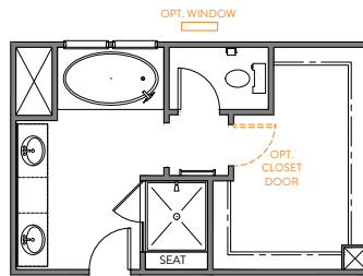
LUXURY BATH OPTION 6 42" x 72" GARDEN TUB w/CERAMIC TUB SURROUND 42" x 48" FRAMED TILE SHOWER BASE TILE WALLS w/12" TILE SEAT LOSE CUBBY
