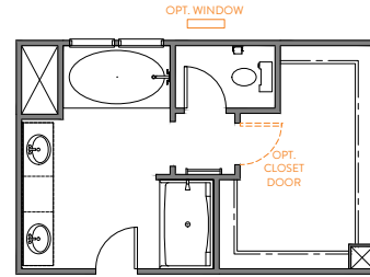
LUXURY BATH OPTION 4 42" x 72" GARDEN TUB 35" x 60" FIBERGLASS SHOWER UNIT LOSE CUBBY
