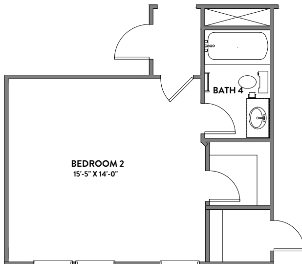
OPT. BATH 4
