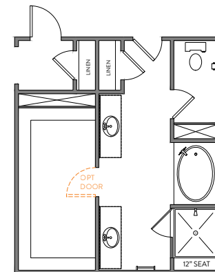
OPT LUXURY BATH 3 42"x60" GARDEN TUB w/CERAMIC TUB SURROUND 42"x48" FRAMED TILE SHOWER BASE TILE WALLS w/12" TILE SEAT
