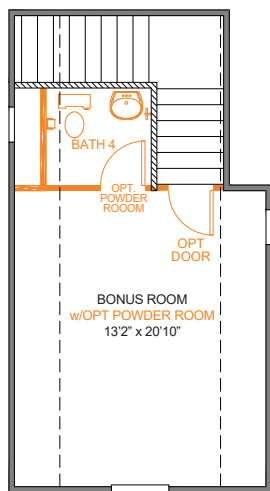
STD BONUS ROOM w/OPT POWDER ROOM
