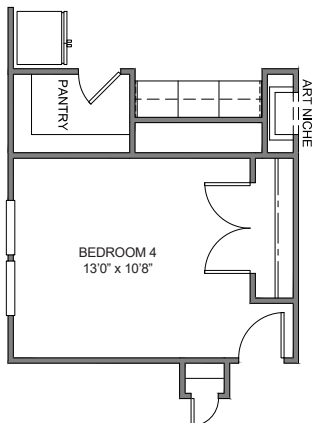
BEDROOM 4 ILO DINING ROOM/STUDY MODIFIES KITCHEN LAYOUT
