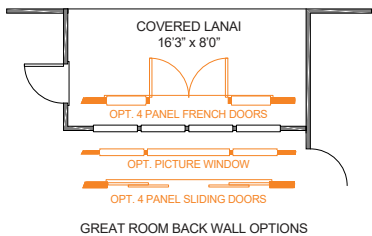
GREAT ROOM BACK WALL OPTIONS
