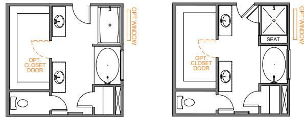
LUXURY BATH 1 42"x60" GARDEN TUB 35"x60" FIBERGLASS SHOWER UNIT
