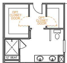
LUXURY SHOWER 2 42"x48" FRAMED TILE SHOWER BASE TILE WALLS w/12" TILE SEAT
