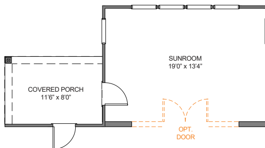
EXTENDED SUNROOM w/COVERED PORCH
