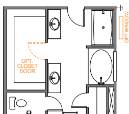
LUXURY BATH 1 42"x60" GARDEN TUB 35"x60" FIBERGLASS SHOWER UNIT
