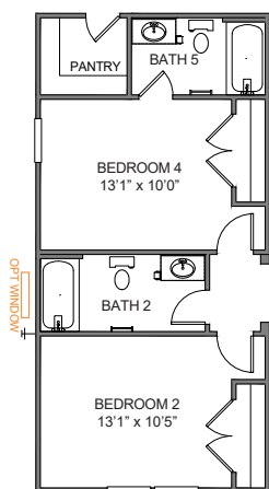
BEDROOM 4 w/FULL BATH ILO DINING ROOM
