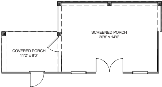
EXTENDED SCREENED PORCH w/COVERED PORCH
