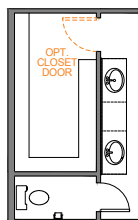
ENLARGED VANITY OPT
