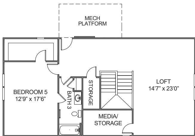
STD GUEST SUITE
