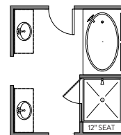
LUXURY BATH OPTION 6 42" x 72" GARDEN TUB w/CERAMIC TUB SURROUND 42" x 48" FRAMED TILE SHOWER BASE TILE WALLS w/12" TILE SEAT
