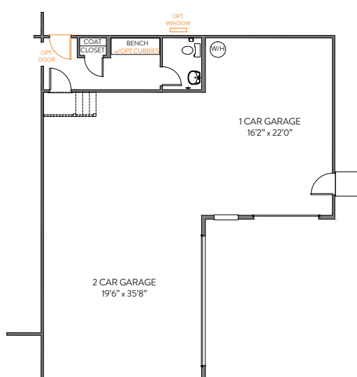
3 CAR FRONT COURTYARD GARAGE w/WINDOW
