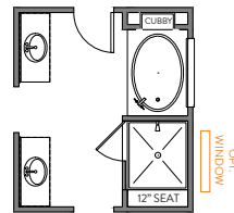
LUXURY BATH OPTION 3 42" x 60" GARDEN TUB w/CERAMIC TUB SURROUND 42" x 48" FRAMED TILE SHOWER BASE TILE WALLS w/12" TILE SEAT
