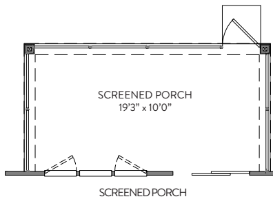
SCREENED PORCH
