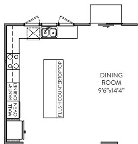
GOURMET KITCHEN
