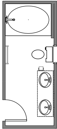
OPT. GARDEN TUB/SHWR (TAKES 9" FROM LAUNDRY)
