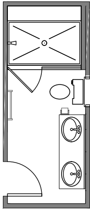
OPT. LUXURY SHOWER 1 (TAKES 9" FROM LAUNDRY)
