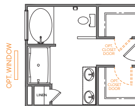
LUXURY BATH 1 42" X 60" GARDEN TUB 35" X 60" FIBERGLASS SHOWER UNIT TAKES 5" FROM BEDROOM 3
