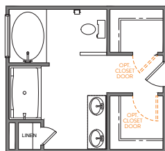
LUXURY BATH 1 42" X 60" GARDEN TUB 35" X 60" FIBERGLASS SHOWER UNIT TAKES 5" FROM BEDROOM 3
