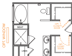
LUXURY BATH 3 42" X 60" GARDEN TUB w/CERAMIC TUB SURROUND 42" X 48" FRAMED TILE SHOWER BASE TILE WALLS w/12" TILE SEAT TAKES 5" FROM BEDROOM 3
