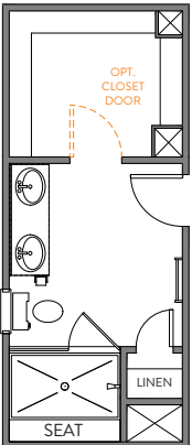
LUXURY SHOWER LOSE 37" FROM CLOSET
