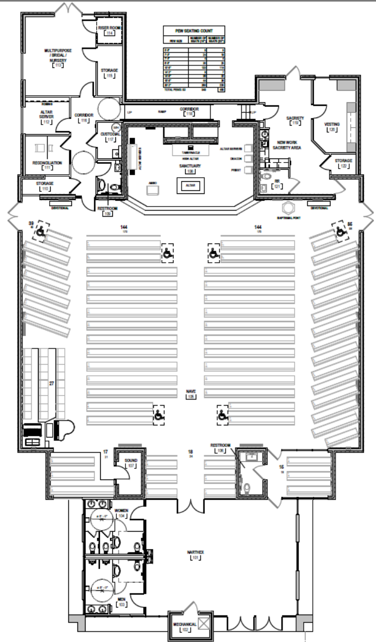
1 FLOOR PLAN - RENOVATION 316' x 147'
