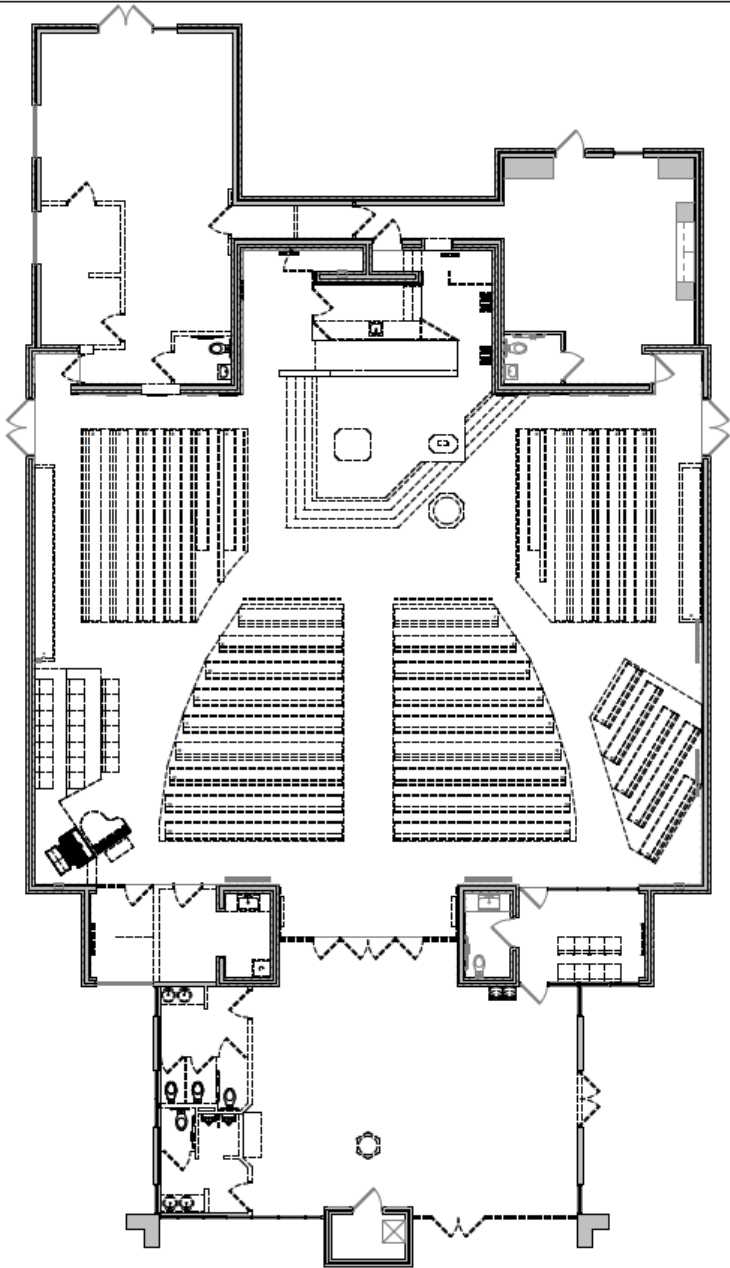
2 FIRST FLOOR PLAN - DEMOLITION 316' x 147'
