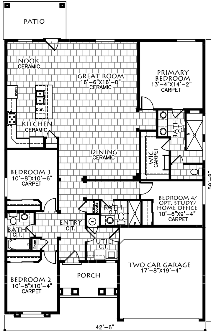
FLOOR PLAN
