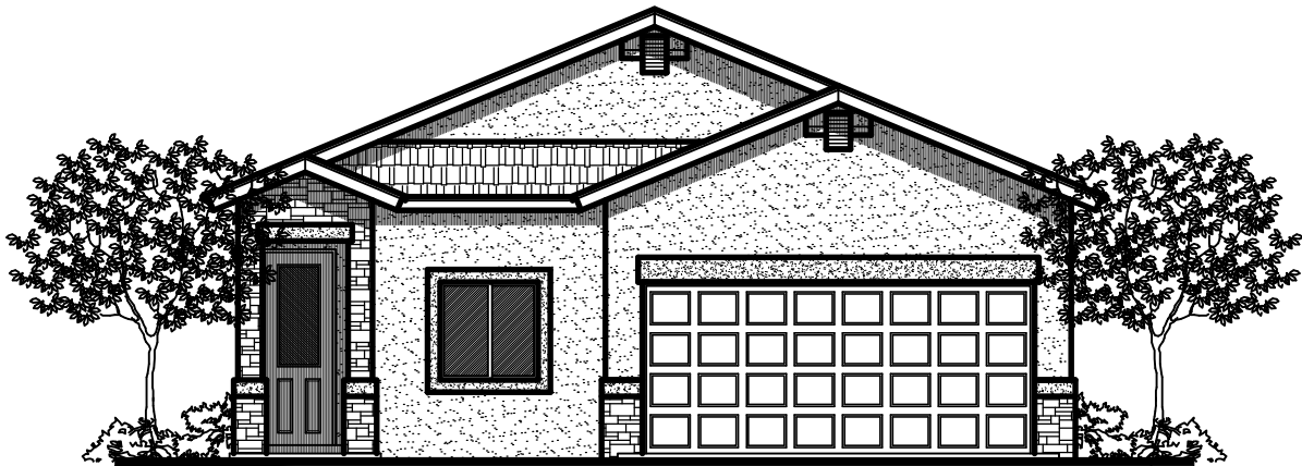
C - ELEVATION (CULTURED STONE)
