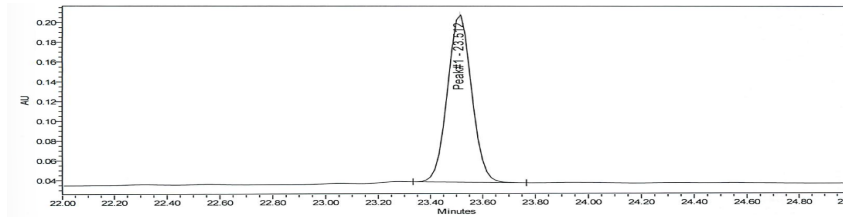
HPLC-MS Chromatogram
