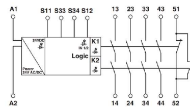
Figure 3 Block diagram
