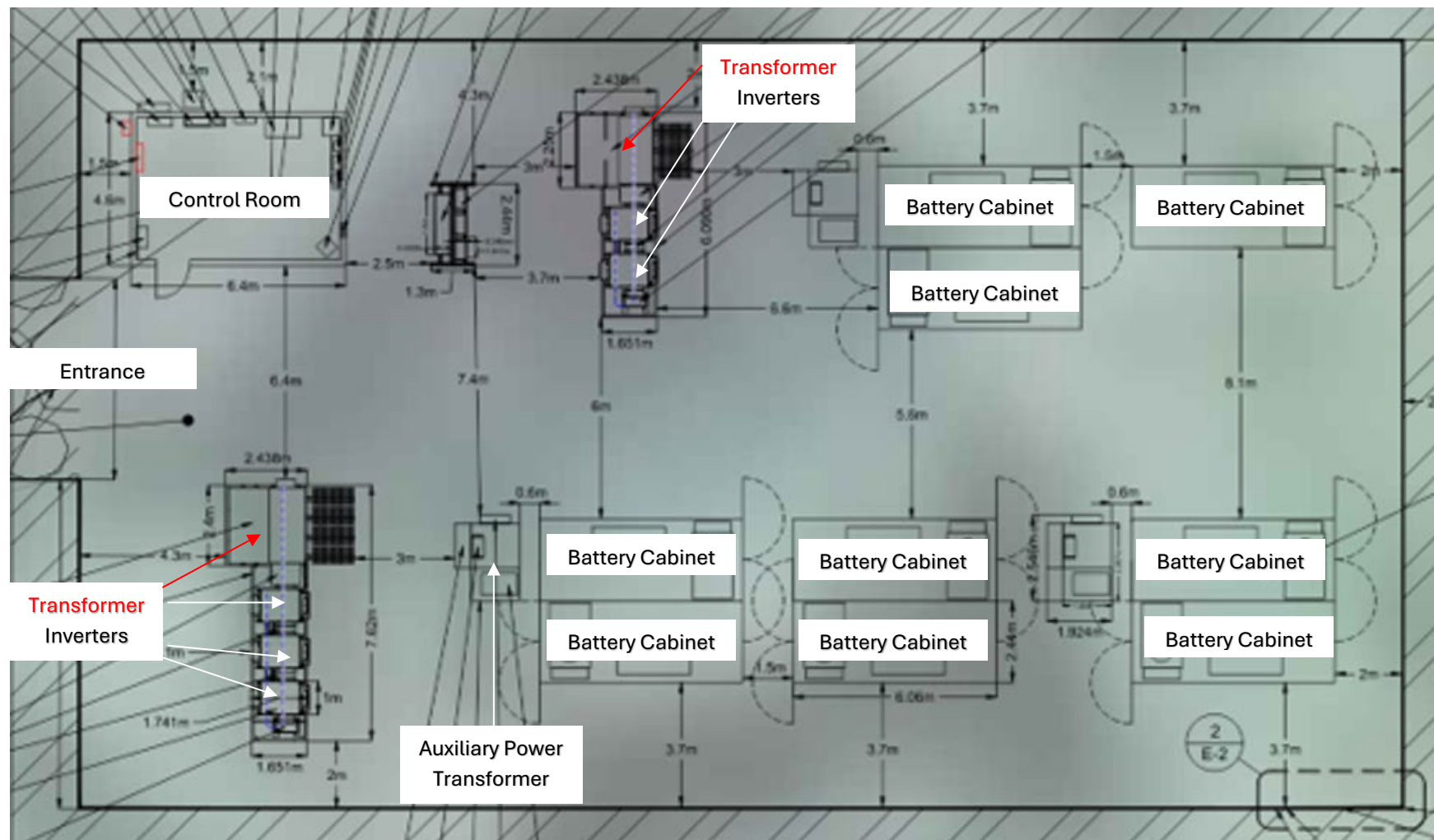
Figure 2. Facility Layout
