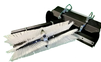
AXI® roller brush with collection bin
