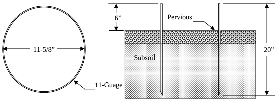
Figure 6: Single-Ring Infiltrometer
