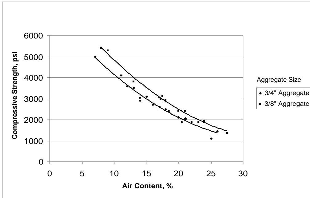
Figure 2.1.6 Compressive Strength vs Air Content
