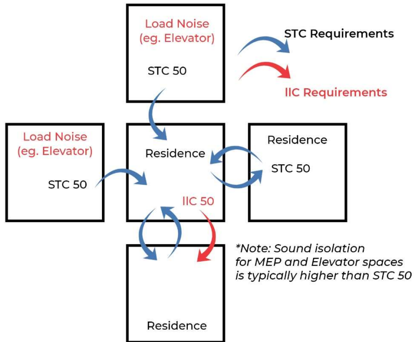
FIGURE 1. Potential Adjacencies in a Residential Building – STC & IIC Requirements
