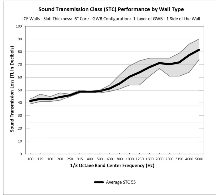
FIGURE 3. Concrete Wall Assemblies – Acoustics Performance Interactive Graph
