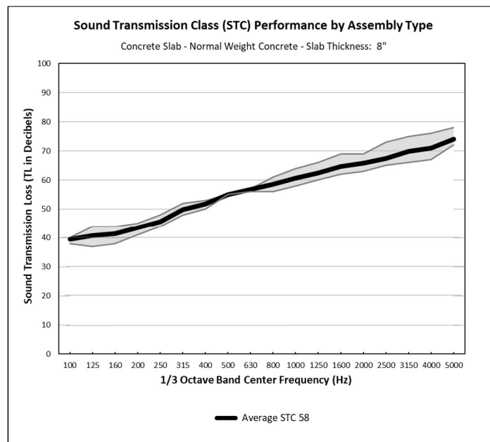
FIGURE 2. Concrete Floor-Ceiling Assemblies – Acoustics Performance Interactive Graph
