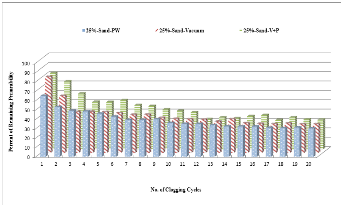
Figure 52. Sand specimens, 25 percent porosity, cleaned by three rehabilitation methods
