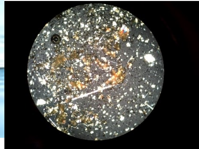
Forensic Dust Testing Fiber ID by Polarizing Light Microscopy
