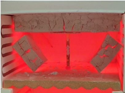
Product Failure Testing Cement Fiber Release After Furnace
