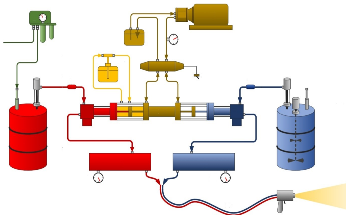
Figure 2: Schematic of a High-Pressure SPF
