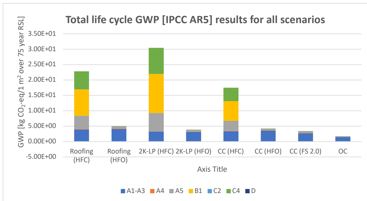
Figure 15: Total life cycle GWP [IPCC AR5] results for all scenarios
