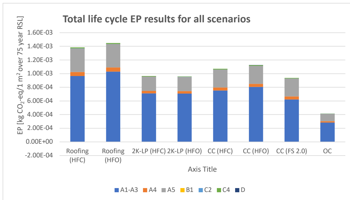
Figure 17: Total life cycle EP results for all scenarios
