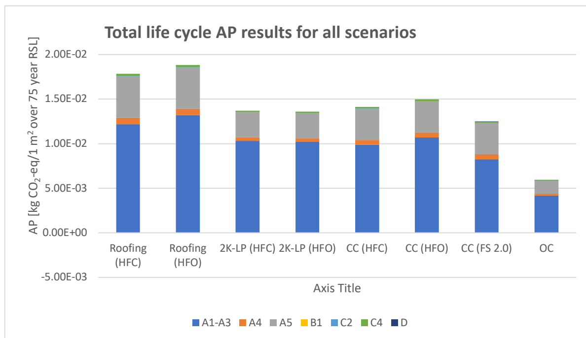
Figure 16: Total life cycle AP results for all scenarios
