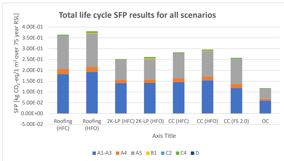
Figure 18: Total life cycle SFP results for all scenarios
