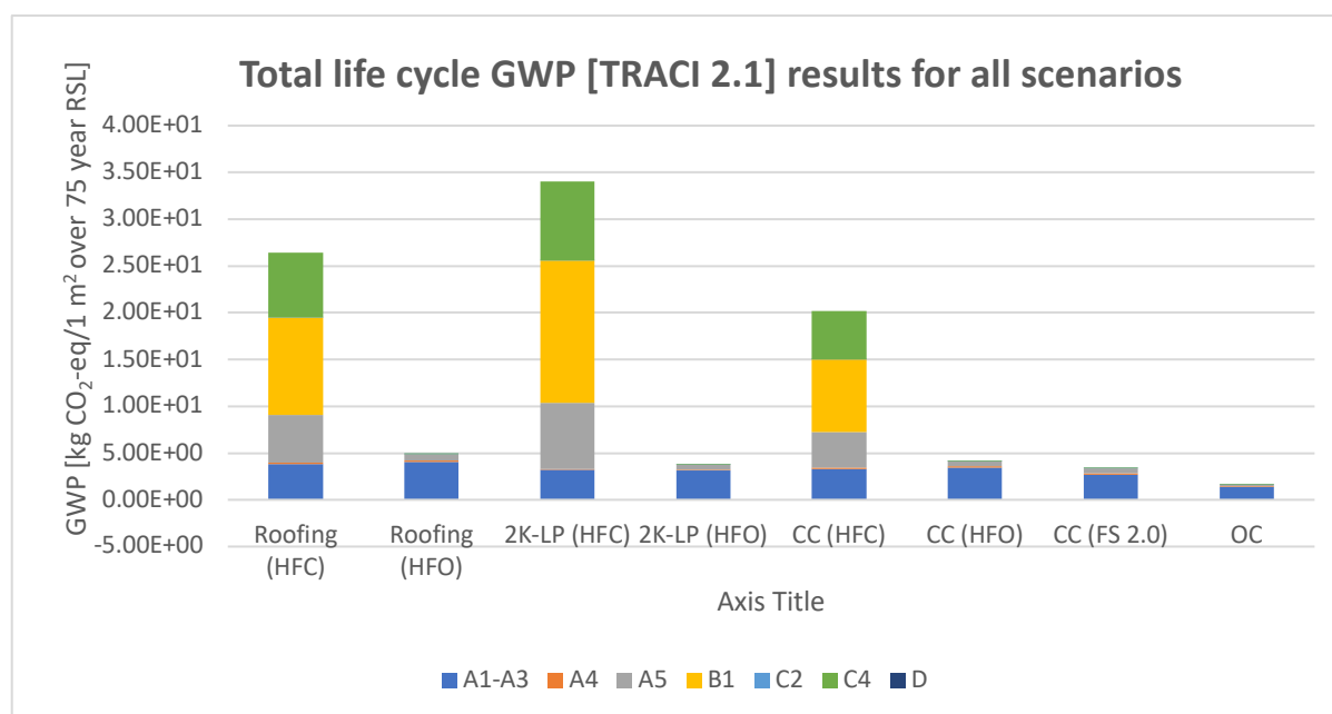
Figure 14: Total life cycle GWP [TRACI 2.1] results for all scenarios
