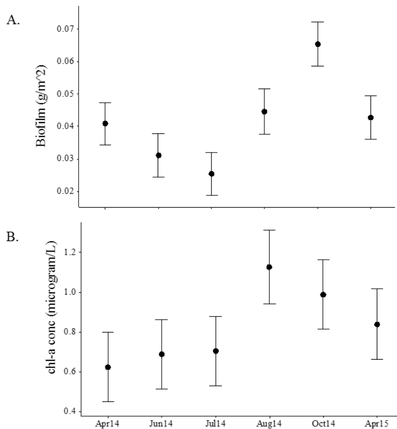
Figure 5: Interval plots of the (A) biofilm organic matter estimate ( \text{g/m}^2 ) and (B) chl- a concentrations ( \mu\text{g/L} ). The black dots represent the average recorded value for this resource and bars are 95% Cis for that data point.
