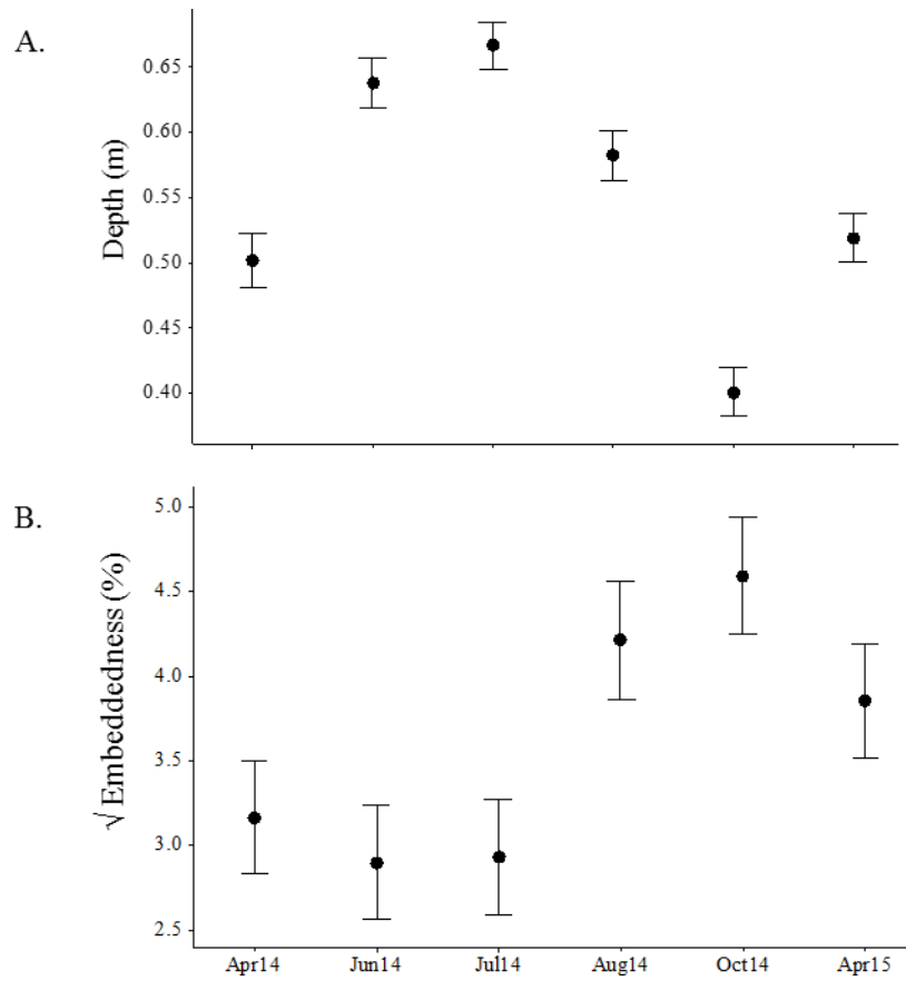
Figure 4: Interval plot for physical habitat parameters, (A) Depth and (B) % Embeddedness, for Rapid Creek based on sampling date. The black dots represent the average recorded value for this variable and bars are 95% Cis for that data point. Embeddedness data \sqrt{\text{-transformed}} to obtain equal variance.
