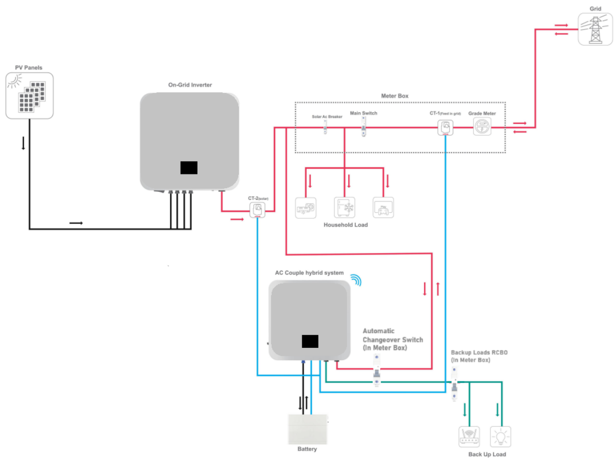
AC Coupled System 1
