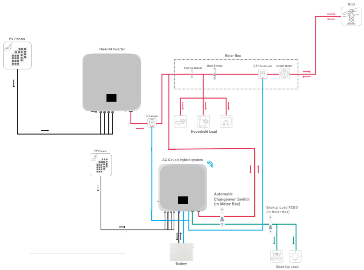
Ac Coupled System 2
