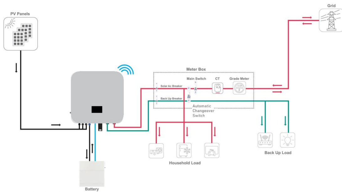
DC Coupled System
