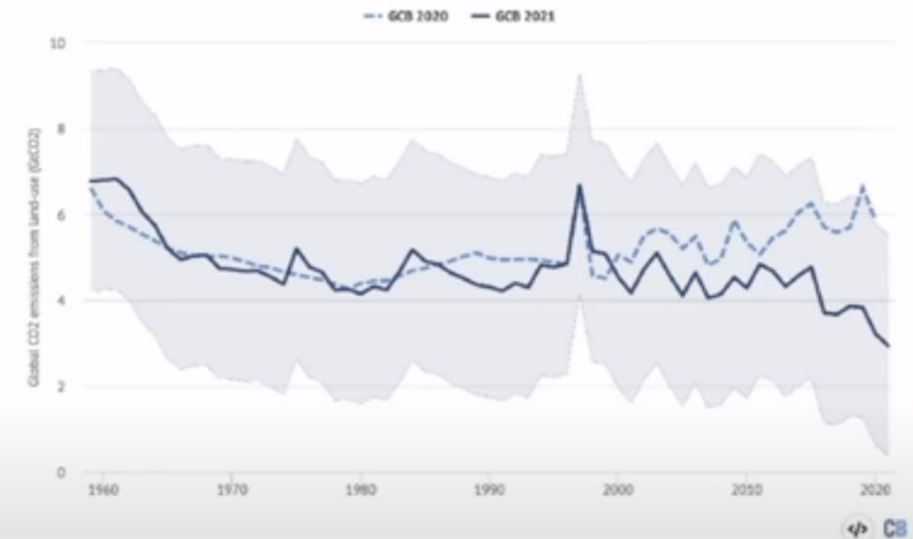
Major downward revision in land-use emissions over the past decade
