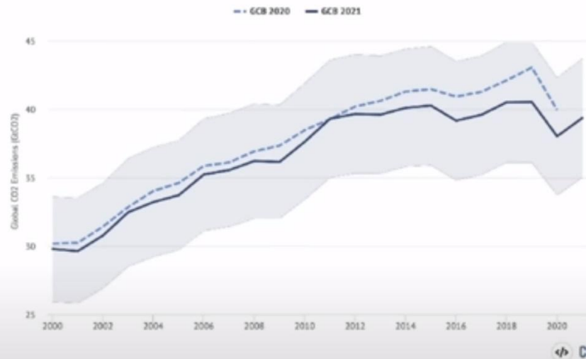
Recent global CO 2 emissions revised notably downward
