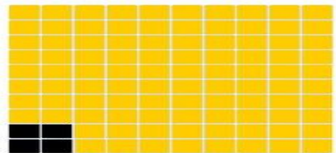
Carbon Dioxide
