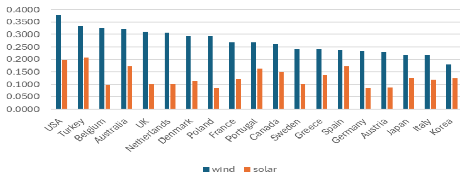
Capacity Factors (CF) for Wind and Solar, 2023
