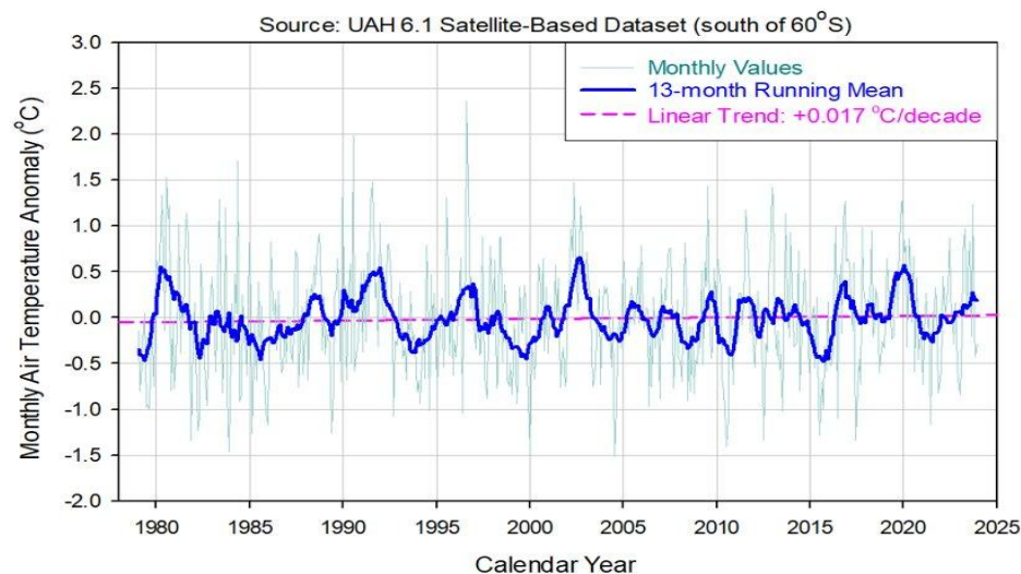
Lower-Troposphere Temperature Anomaly over Antarctica: 1979 - 2023
