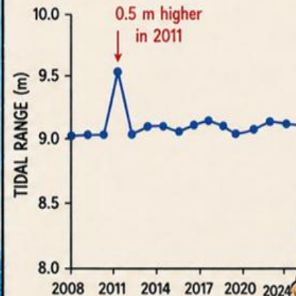
JERSEY: HIGH TIDAL RANGE (2008–2024)
