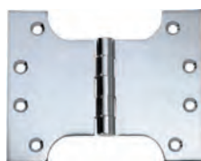
2681 CP (W125xH100xT4mm)
