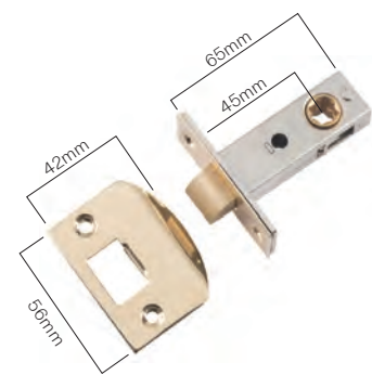
9570 PB B45mm
