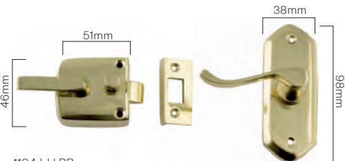
P40mm
