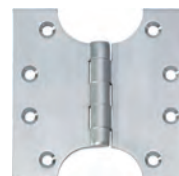
2780 SC (W100xH100xT4mm)
