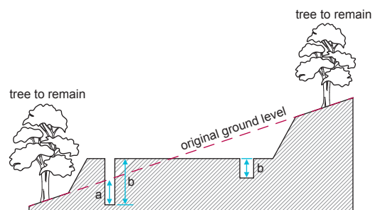
Figure 1: Levels from which foundation depths are measured where trees or hedgerows are to remain
