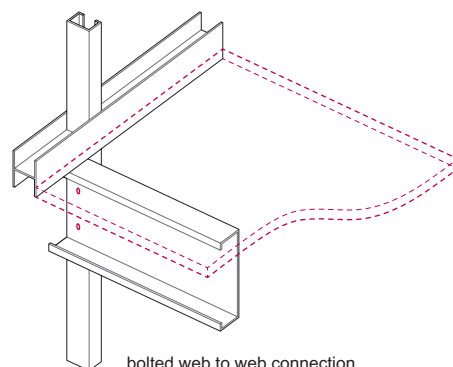
bolted web to web connection
