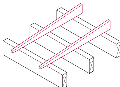
Solid or engineered joists Furrings fixed perpendicular to joists
