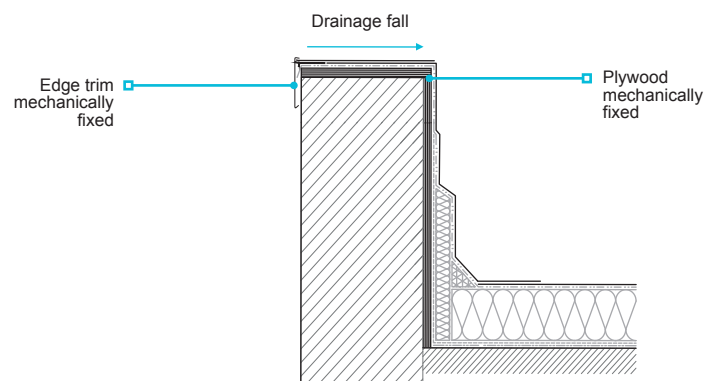
Parapet detail with waterproofing taken over top of wall and finished with an edge trim
