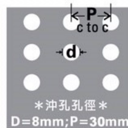
型號.4H-1848P
