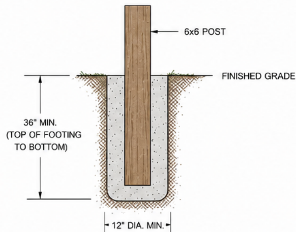
POST FOOTING DETAIL
