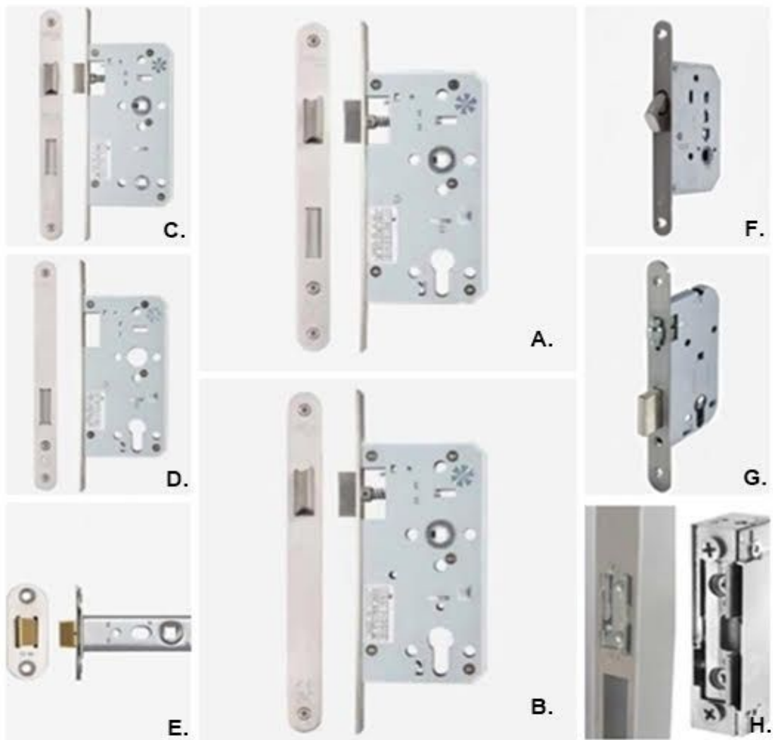
Locking Types.
