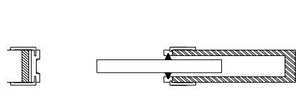
Scorrevole scomparsa _Pocket sliding NTCPKVSM
