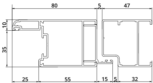
SPORTELLLO PANEL
