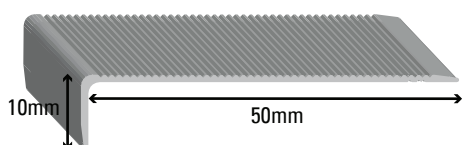
#340 – Universal Compliant Stair
