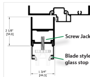
WIDE STILE
