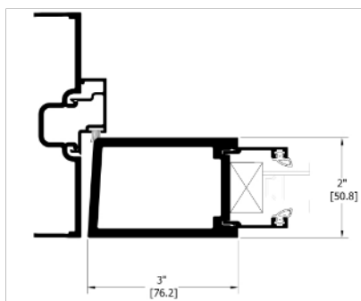
NARROW STILE
