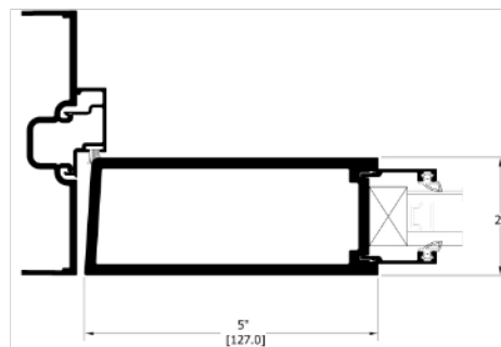
WIDE STILE
