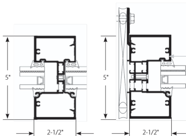
Screw Spline Frame Construction
