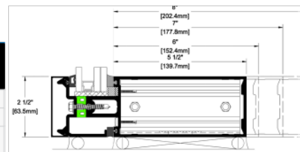
Multiple System Depth Options
