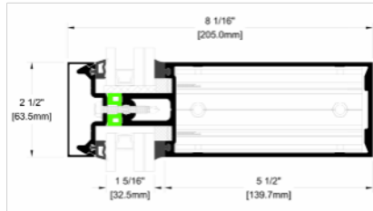
Shear Block Construction
