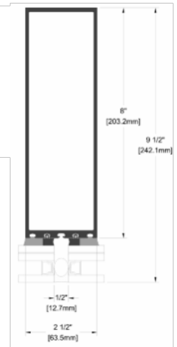
Structural Glazed Horizontals and Verticals
