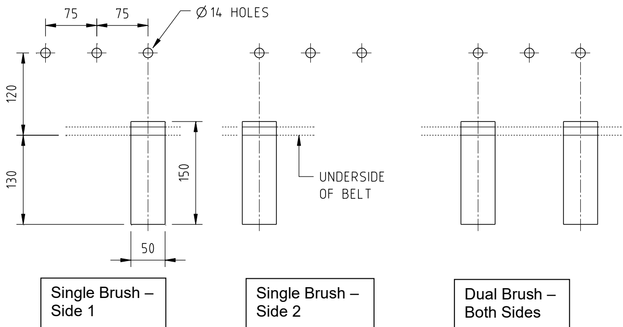
Figure 1 - Installation Positions
