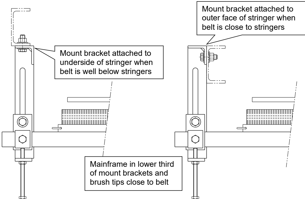
Figure 3 - Mount Brackets
