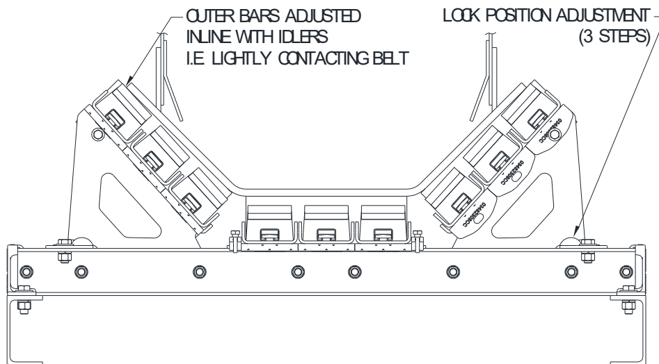
Figure 8 - Wing Adjustment
