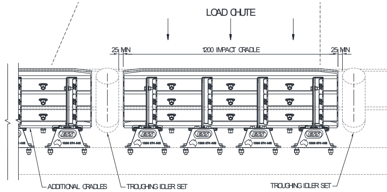
Figure 2 - Modular Impact Cradle Layout
