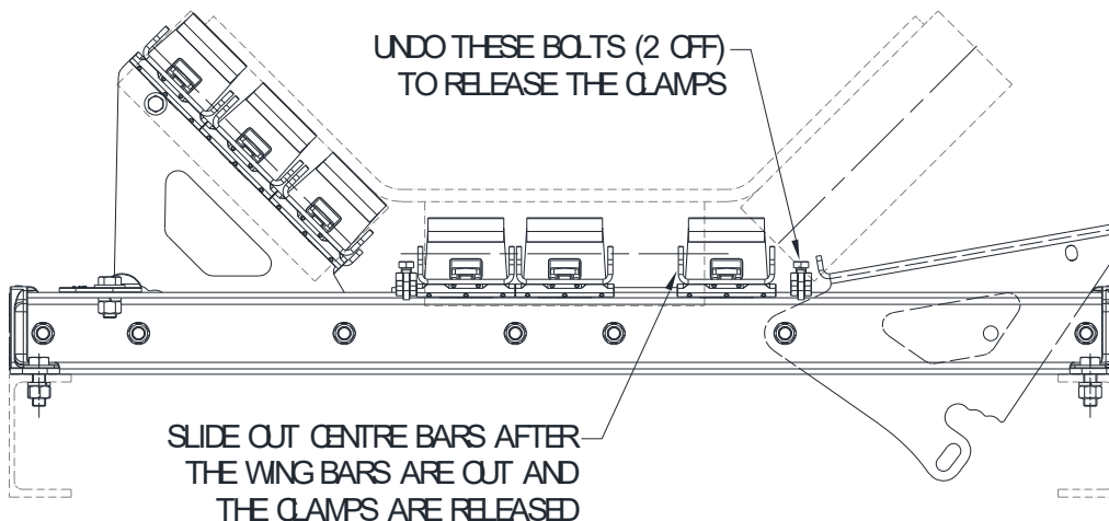
Figure 5 - Sliding Out Centre Bars
