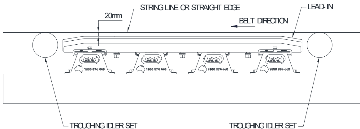
Figure 6 - Cradle Positioning
