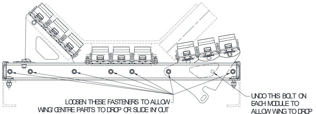
Figure 3 – Lowering Down Wing Sets
