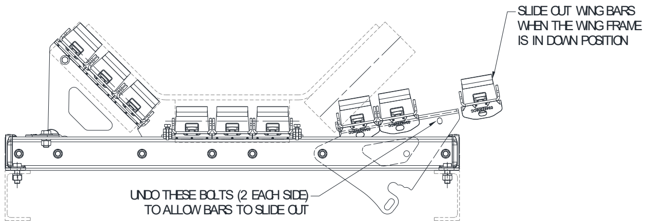
Figure 4 – Sliding Out Wing Bars
