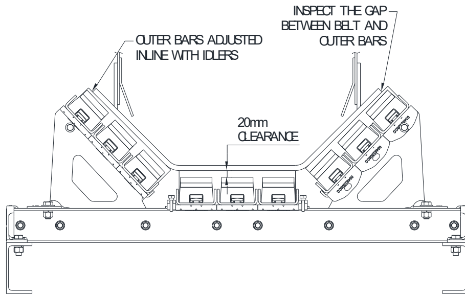
Figure 7 - Cradle Setup Clearances
