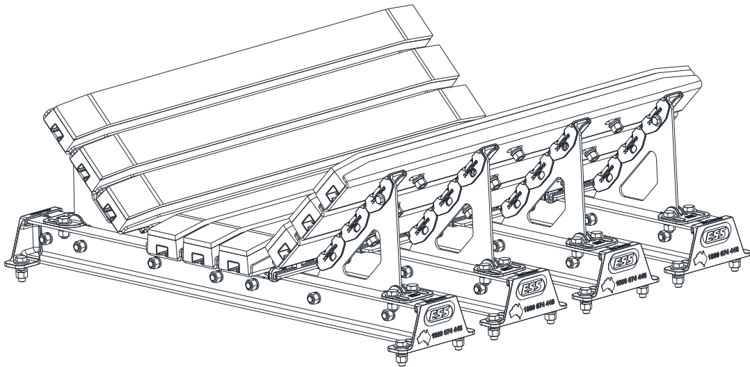
Figure 1 - Complete Impact Cradle Assembly
