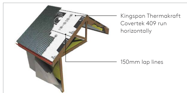
Figure 1. Kingspan Thermakraft Covertex 409 direct fix method.
