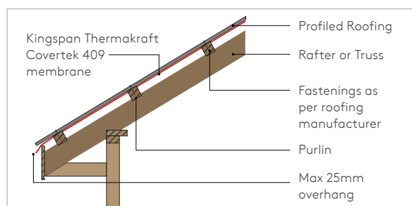
Figure 3. Wooden construction.
