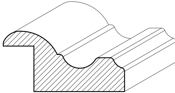
SWPM02 2 \frac{1}{16} " x 1"
