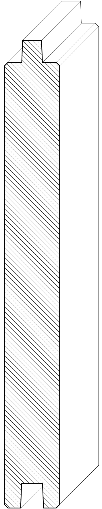
SWFL11 1" \times 8\frac{7}{16}"
