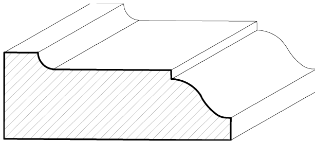
SWOG15 2\frac{1}{4} " x \frac{7}{8} "
