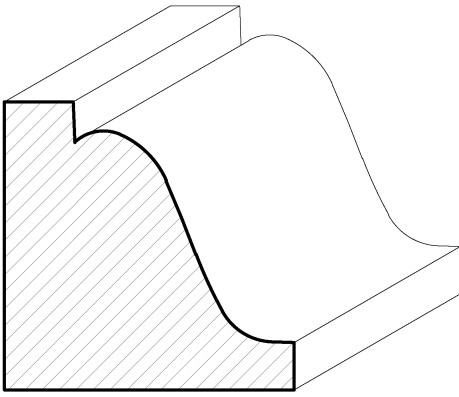
SWOG33 1\frac{1}{2}" \times 1\frac{1}{2}"
