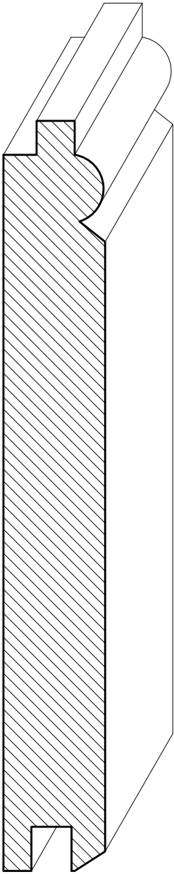
SWPNL07 \frac{3}{4} " x 5\frac{1}{8} " (Face)
