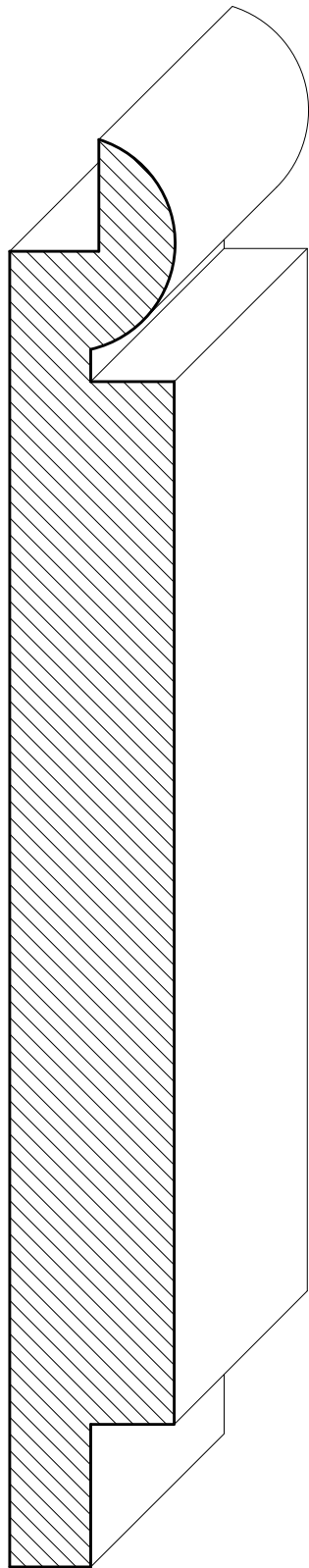
SWSL04 \frac{7}{8} " x ANY WIDTH
