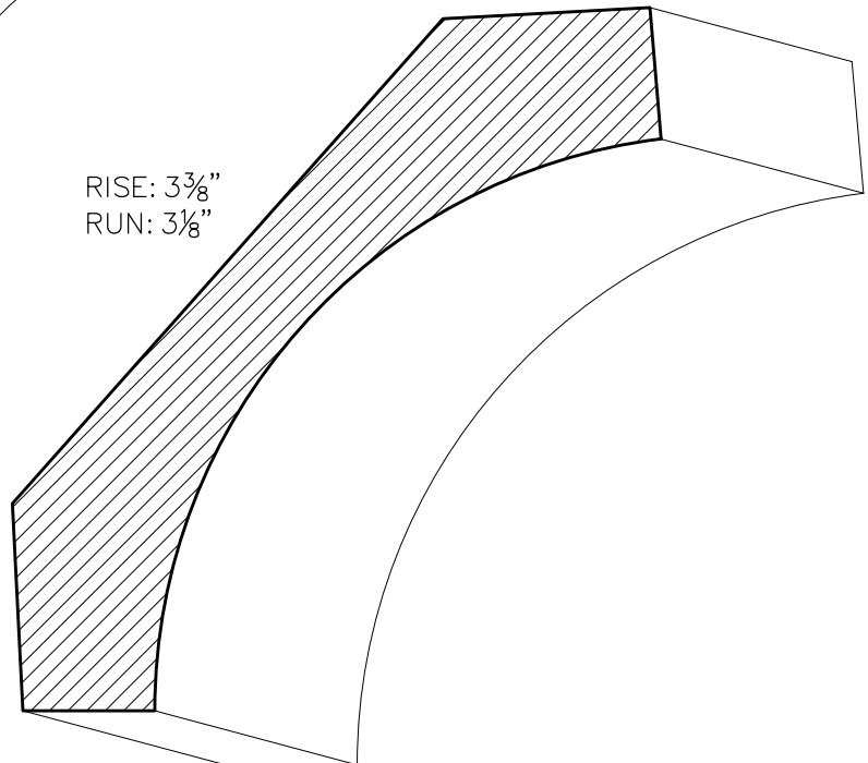
SWCC04 1\frac{3}{8} " \times 4\frac{1}{2} "
