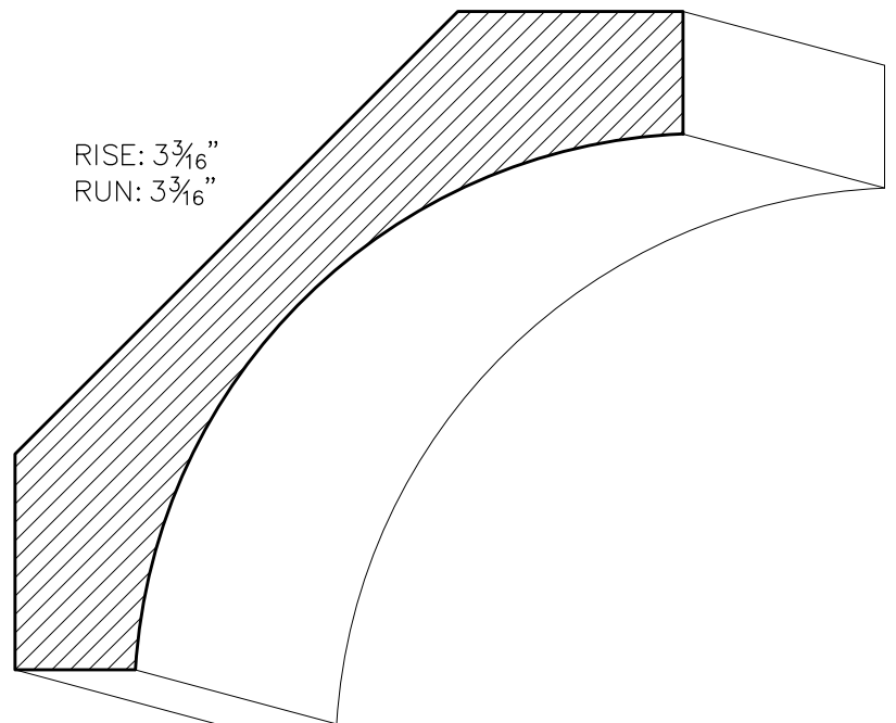
SWCC06 1\frac{1}{4}" \times 4\frac{1}{2}"
