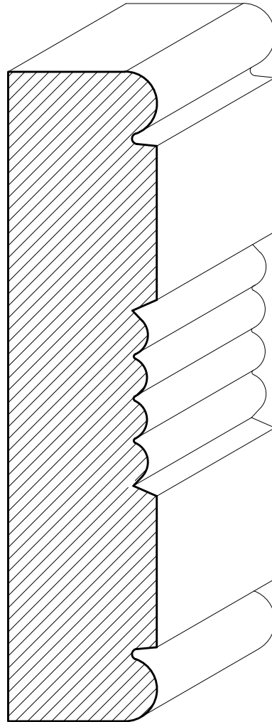
SWCH10 1 \frac{1}{6} " x 4 \frac{3}{4} "
