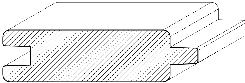
SWFL12 1\frac{5}{16} " x ANY WIDTH
