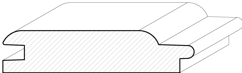
SWFL06 \frac{3}{4} " x 2" (face)
