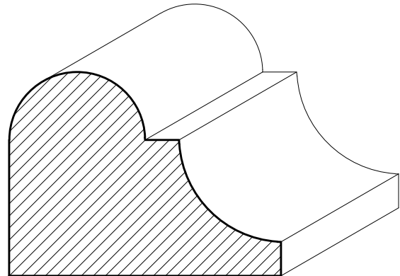
SWCH12 2" x 1 \frac{1}{2} "
