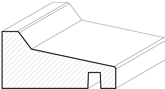
SWMSC10 1\frac{15}{16}" \times 1"
