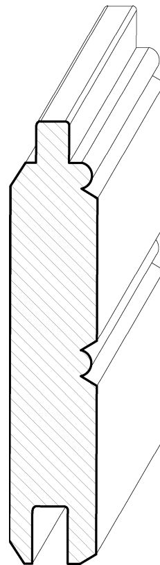
SWPNL18 \frac{5}{8}" \times 3\frac{5}{16}"
