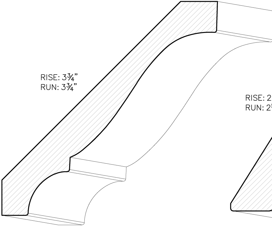
SWCR33 1\frac{1}{16}" \times 5\frac{5}{16}"
