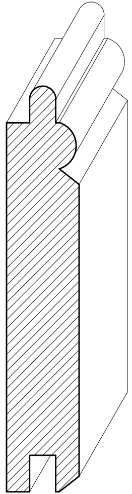
SWPNL15 \frac{3}{4} " x 3" (Face)
