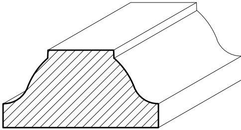
SWCH13 1\frac{5}{8}" \times 1\frac{3}{16}"
