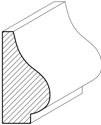
SWCP11 1\frac{3}{16}" \times 1\frac{1}{2}"
