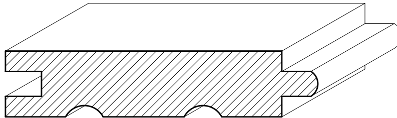
SWFL03 (EXTERIOR T & G) 1\frac{3}{8} " x 2\frac{7}{8} " (Face)
