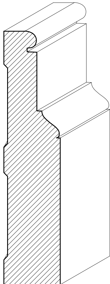
SWCA17 1" \times 4\frac{1}{2}"
