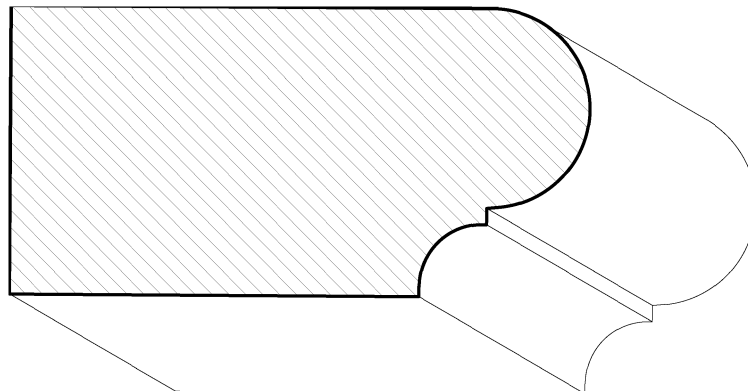
SWWS01 3" x 1½"
