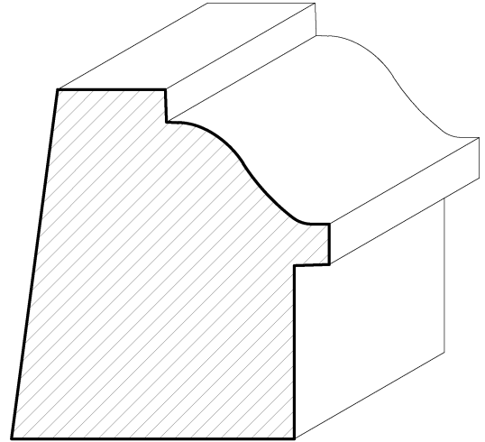
SWBB10 1\frac{13}{16}" \times 2"
