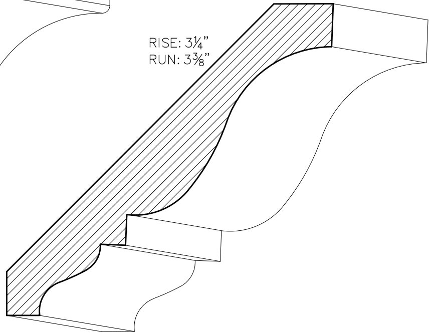
SWCR51 \frac{3}{4}" x 4 \frac{1}{16}"
