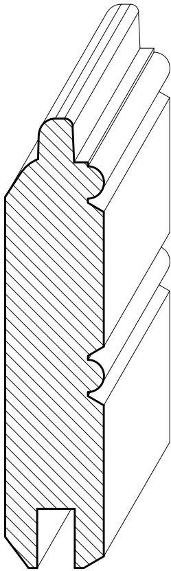
SWPNL10 \frac{3}{4} " x 3" (Face)
