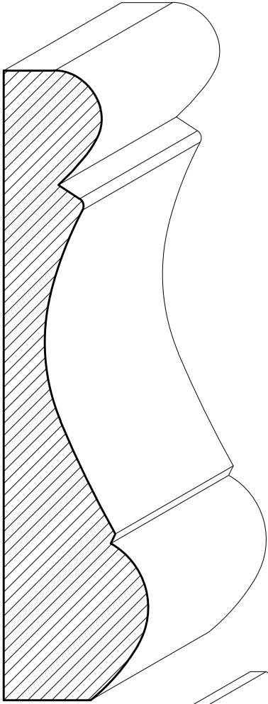
SWCA18 1" x 4 \frac{5}{8} "
