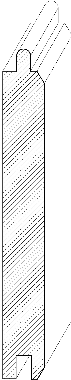
SWPNL02 \frac{3}{4} " x 5\frac{1}{8} " (Face)
