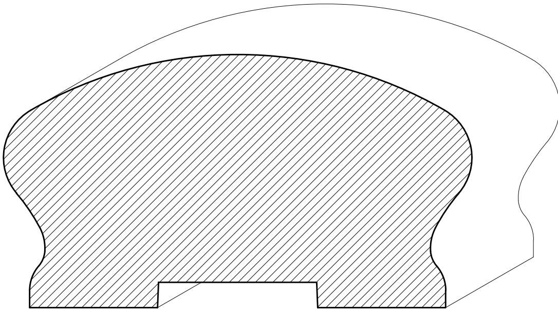
SWHR01 4\frac{3}{4}" \times 2\frac{5}{8}"
