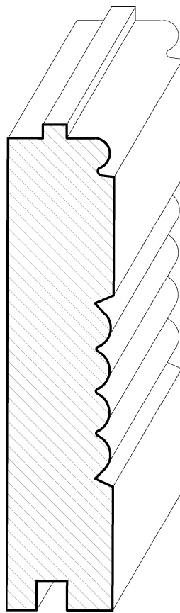
SWPNL17 \frac{3}{4}" \times 3\frac{7}{16}"
