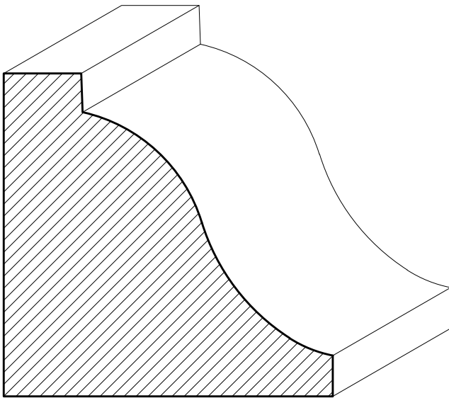
SWOG03 2\frac{7}{16}" \times 2\frac{3}{8}"
