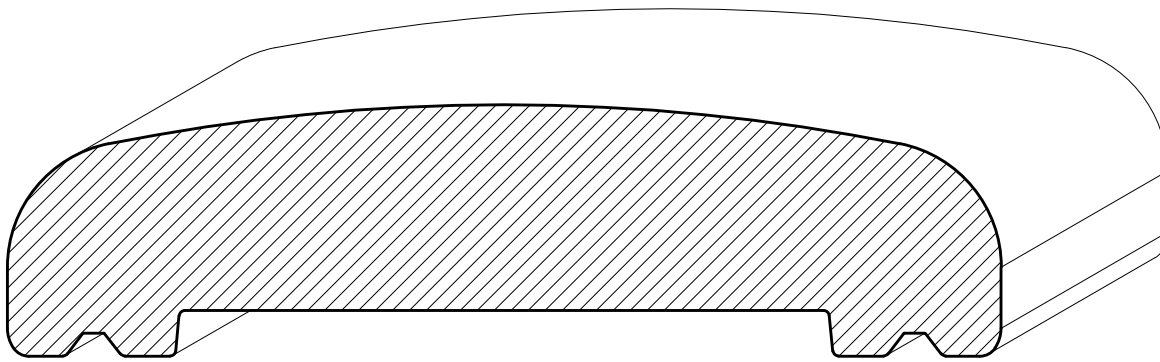
SWHR13 5¼" x 1¼"
