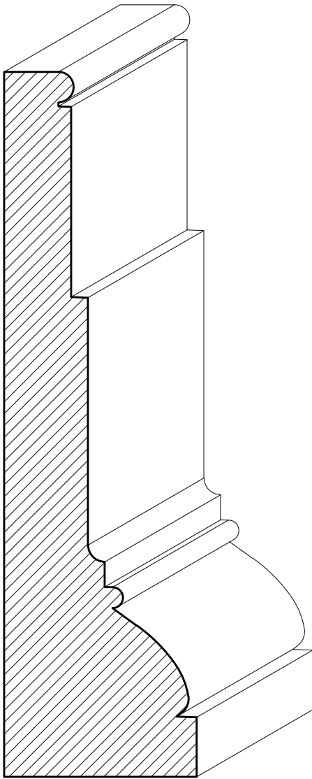
SWCA27 1\frac{7}{16}" \times 5\frac{1}{4}"
