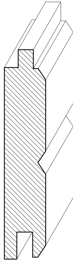
SWPNL06 \frac{3}{4}" \times 3" (Face)
