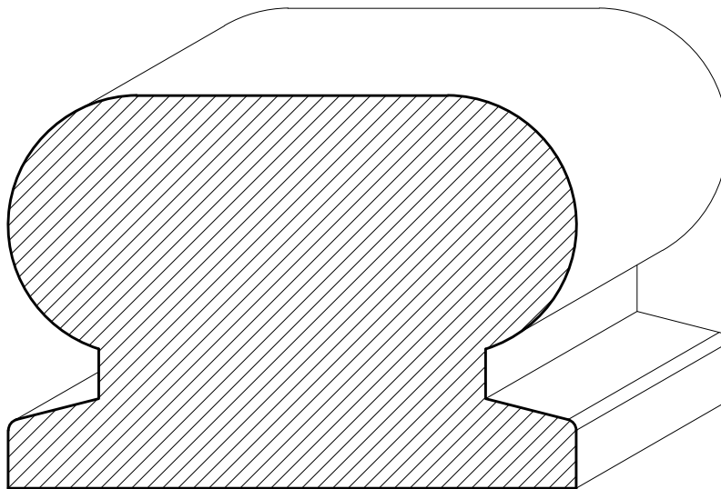
SWHR02 3\frac{1}{4}" \times 2\frac{1}{4}"
