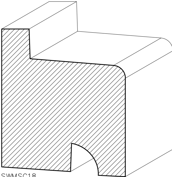
SWMSC18 2 \frac{1}{4} " x 2 \frac{1}{16} "
