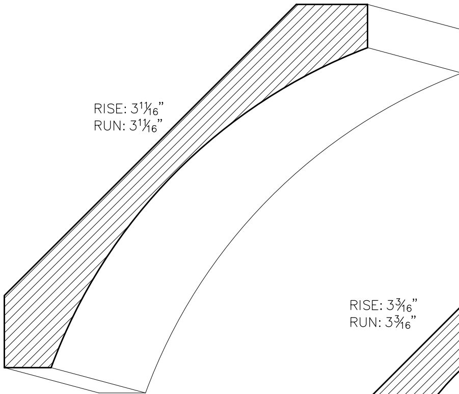
SWCC05 \frac{7}{8}" \times 5\frac{1}{4}"
