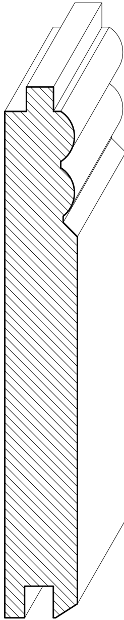
SWPNL08 \frac{3}{4} " x 5\frac{1}{6} " (Face)
