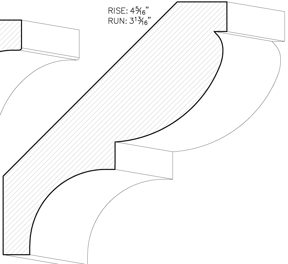
SWCR36 1\frac{1}{2}" \times 5\frac{3}{4}"
