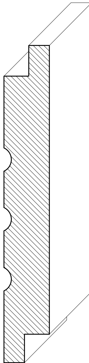
SWSL05 \frac{3}{4} " x ANY WIDTH
