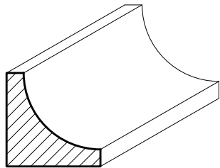
SWQR04 1\frac{1}{16}" \times 1\frac{1}{16}"
