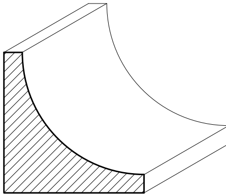
SWQR05 1\frac{7}{16}" \times 1\frac{7}{16}"
