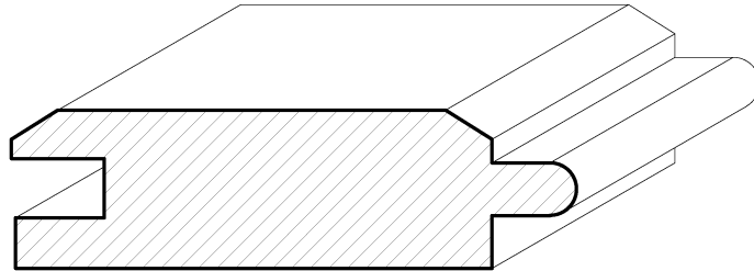
SWFL05 \frac{3}{4} " x 1\frac{3}{4} " (face)
