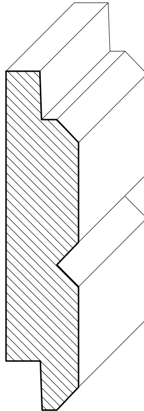
SWSL18 \frac{3}{4}" \times 3\frac{1}{2}"
