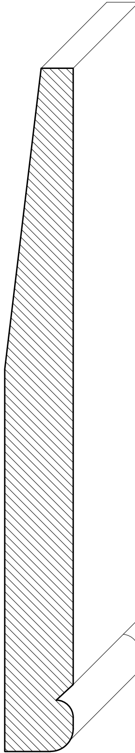
SWSI09 \frac{3}{4}" \times 7\frac{5}{16}"
