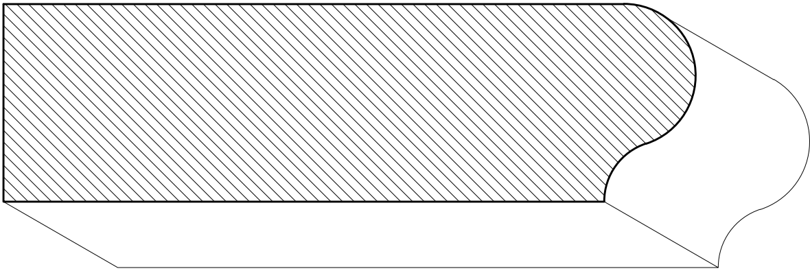
SWWS09 5¼" x 1½"
