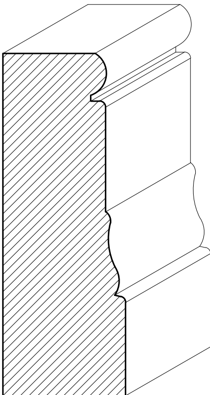
SWCA13 1\frac{1}{4}" \times 3\frac{1}{2}"
