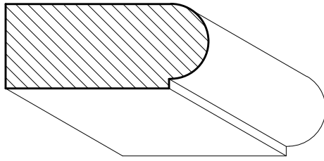
SWWS08 1\frac{1}{2}" \times \frac{5}{8}"
