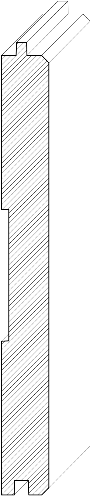
SWFL08 1\frac{3}{16}" \times 7\frac{1}{4}" (face)
