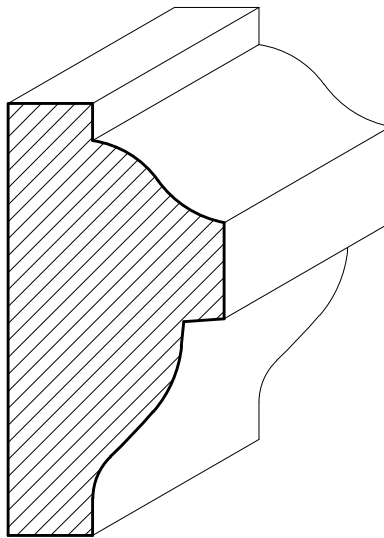
SWCH02 1⅛" x 2¼"
