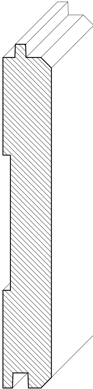
SWFL09 1\frac{3}{16}" \times 5\frac{1}{4}" (face)
