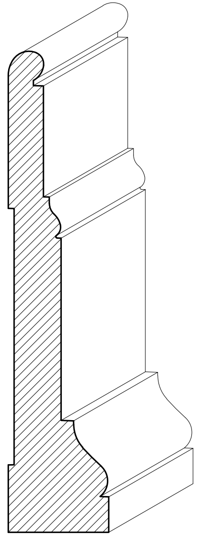
SWCA20 1 \frac{1}{16} " x 5"
