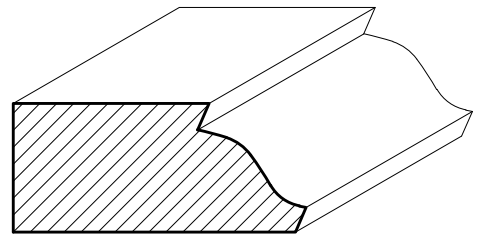
SWOG29 1\frac{1}{2}" \times 1\frac{1}{16}"
