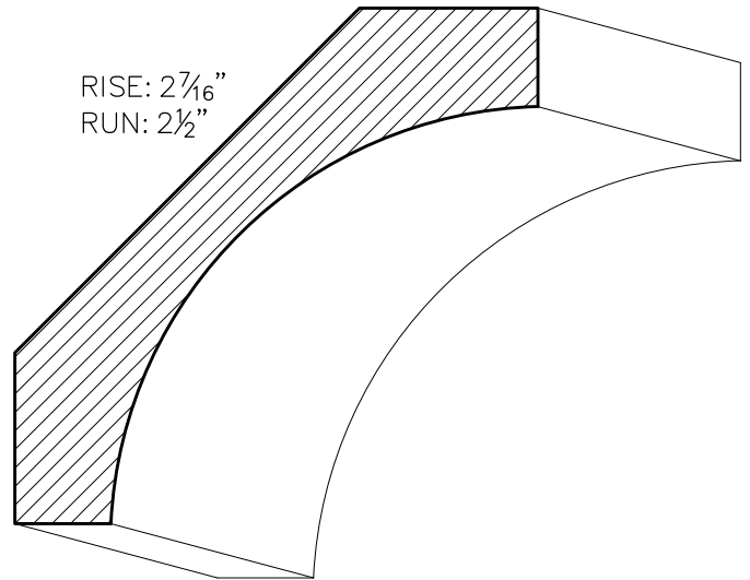
SWCC02 1" \times 3\frac{1}{2} "
