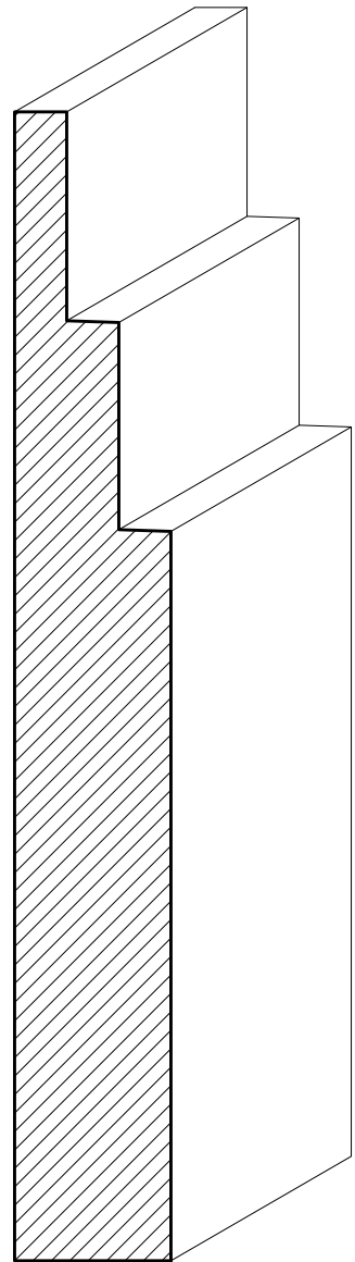
SWBA06 \frac{3}{4}" \times 5\frac{1}{2}"
