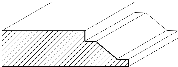
SWOG21 2\frac{1}{4}" \times \frac{5}{8}"
