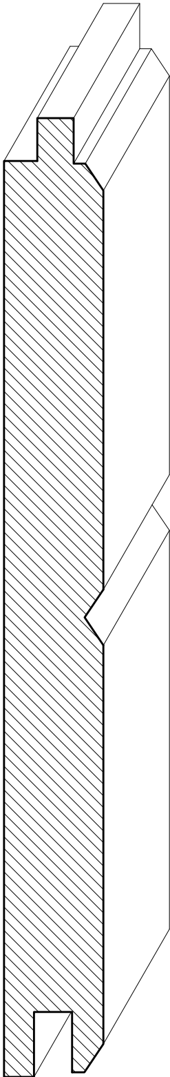
SWPNL04 \frac{3}{4}" \times 6\frac{7}{16}" (Face)
