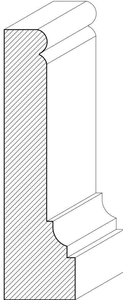
SWCA12 1\frac{1}{4}" \times 4\frac{13}{16}"
