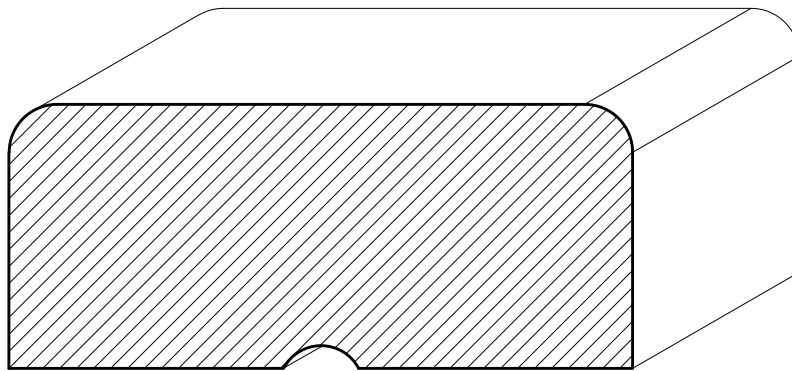
SWDE02 1\frac{3}{8}" \times 3\frac{1}{4}"
