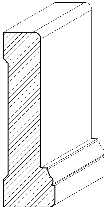
SWCA22 \frac{7}{8} " x 3"
