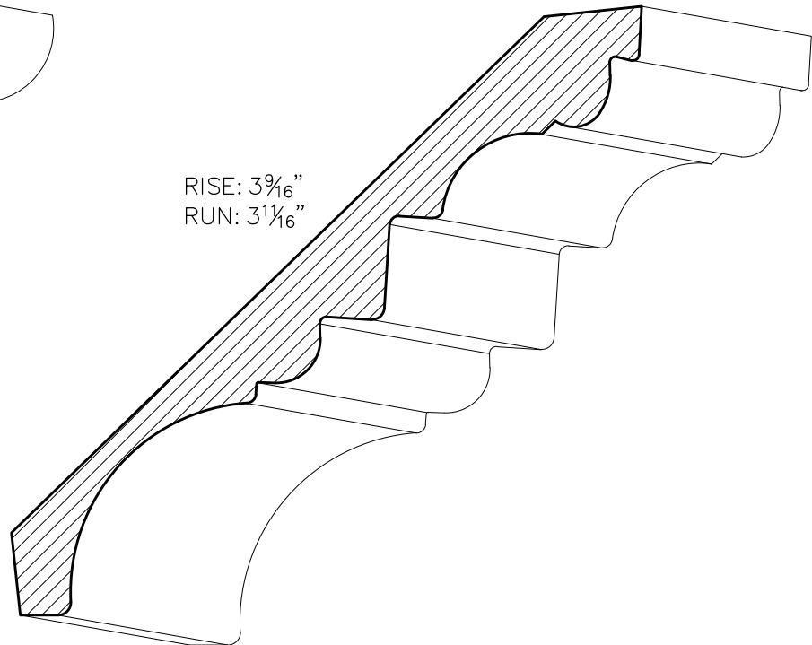
SWCR30 \frac{5}{8}'' \times 5''
