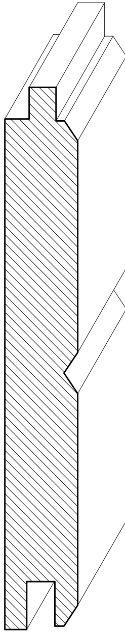
SWPNL05 \frac{3}{4}" \times 4\frac{3}{4}" (Face)
