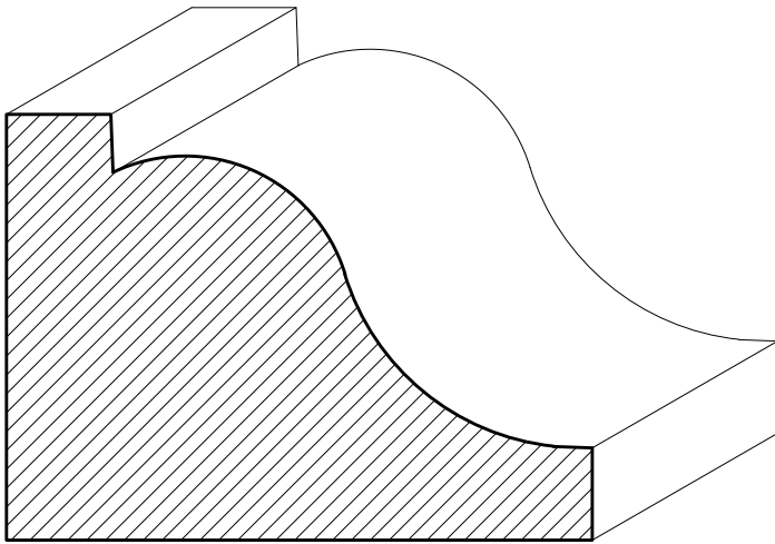
SWOG25 2\frac{3}{4}" \times 2"
