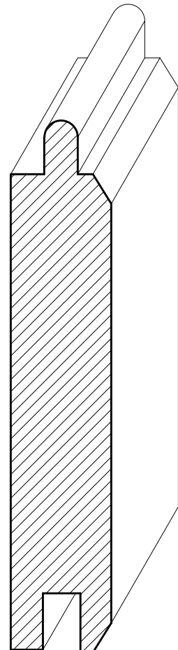
SWPNL03 \frac{3}{4} " x 3\frac{1}{8} " (Face)
