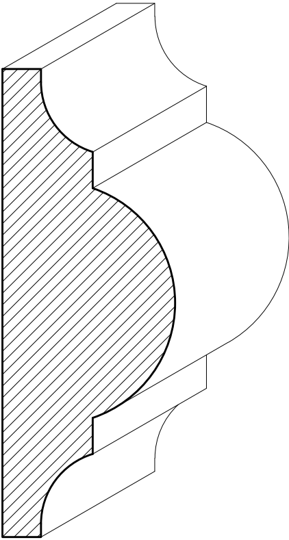
SWCH01 1¼" x 3½"
