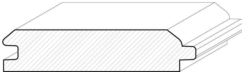
SWFL07 \frac{3}{4} " x 2\frac{3}{4} " (face)
