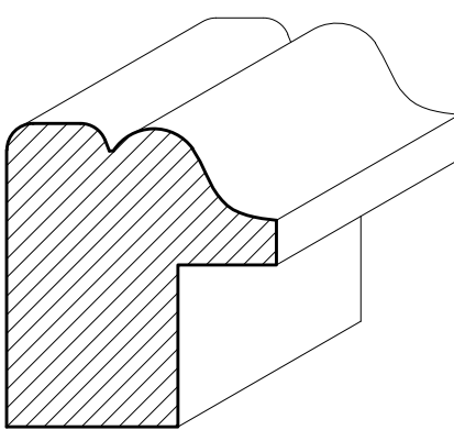
SWBB02 1\frac{7}{16}" \times 1\frac{1}{4}"
