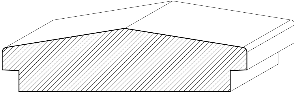
SWHR16 4½" x 1⅛"
