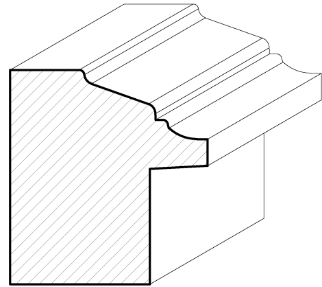
SWBB12 1\frac{1}{2}" \times 1\frac{5}{8}"
