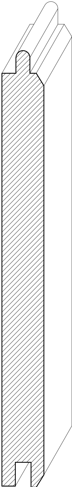
SWPNL01 \frac{3}{4} " x 6\frac{7}{8} " (Face)
