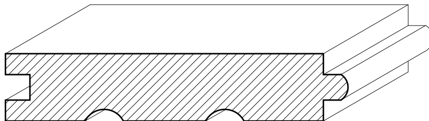
SWFL04 (INTERIOR T & G) 1\frac{3}{8} " x ANY WIDTH
