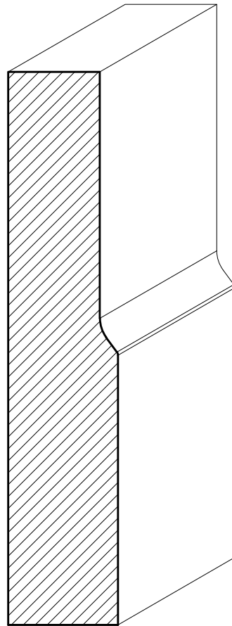
SWBA12 1\frac{3}{16}" \times 4\frac{1}{8}"
