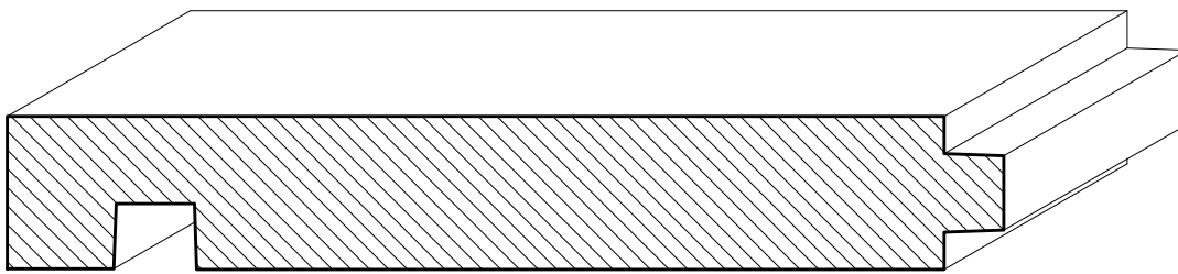
SWCB05 4\frac{1}{16}" \times \frac{3}{4}"
