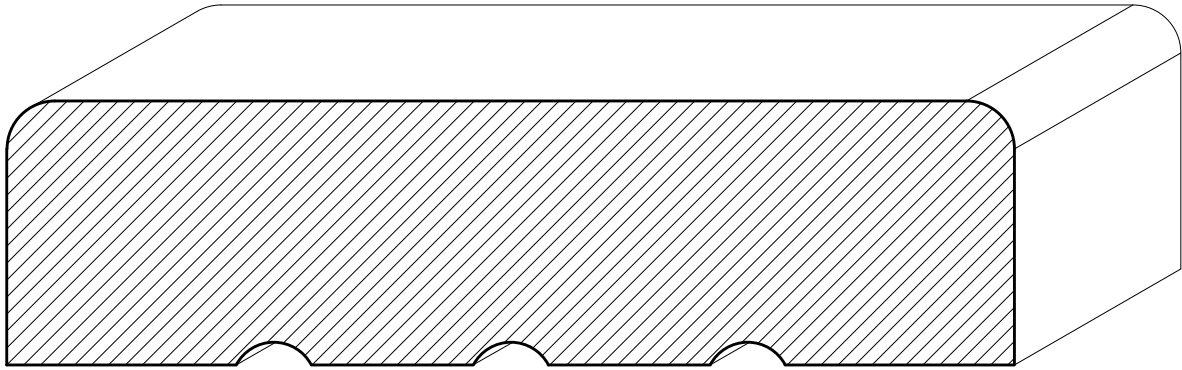
SWDE01 1\frac{3}{8}" \times 5\frac{1}{4}"
