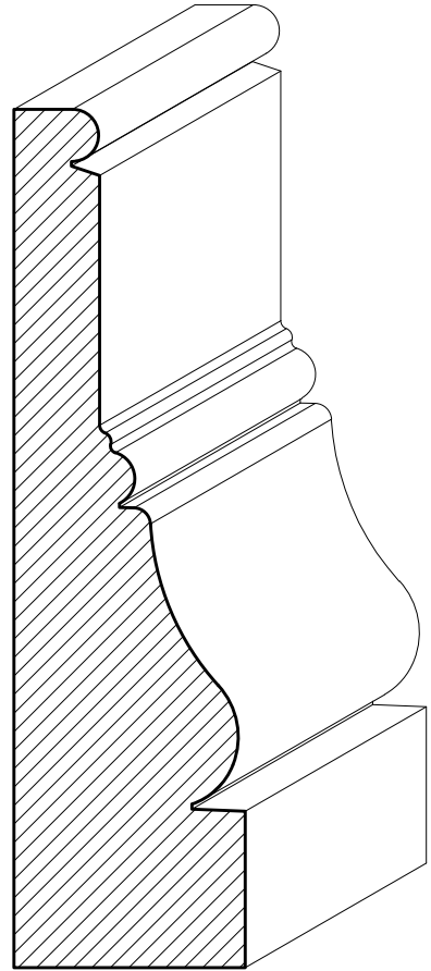
SWCA28 1\frac{1}{8}" \times 4\frac{1}{8}"
