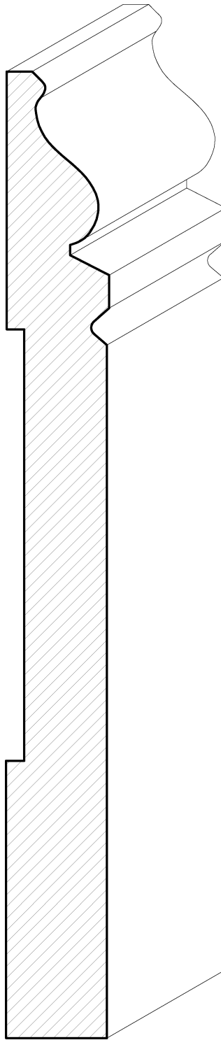
SWBA02 \frac{3}{4} " x ANY WIDTH
