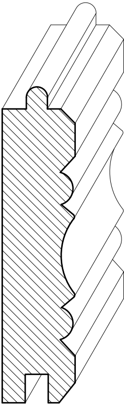
SWPNL13 \frac{3}{4} " x 3" (Face)
