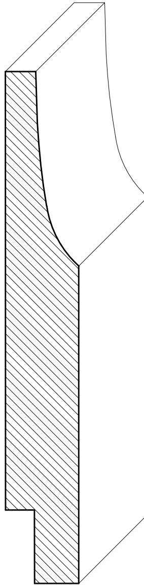
SWSI05 \frac{3}{4}" \times 5\frac{1}{4}"
