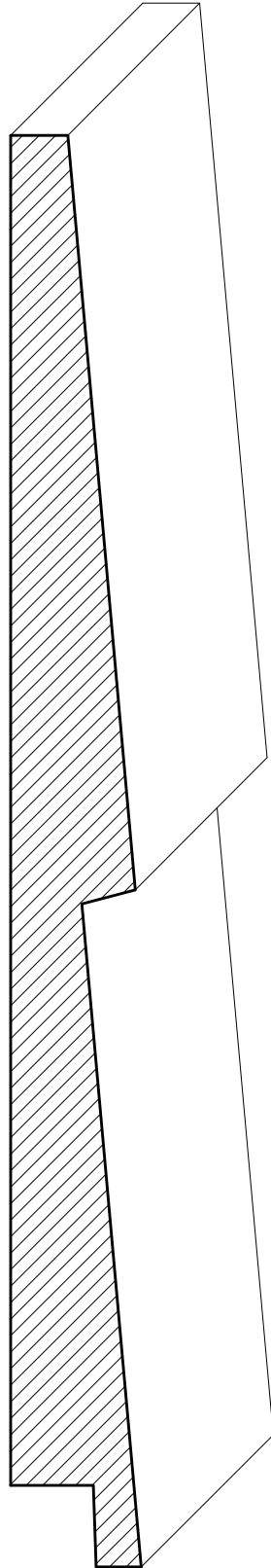
SWSL11 \frac{3}{4}" \times 7\frac{3}{4}"
