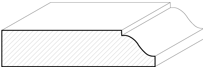
SWOG37 2\frac{1}{2}" \times \frac{5}{8}"
