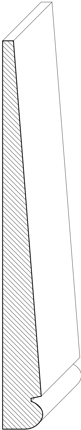
SWSI06 \frac{3}{4} " x 7"
