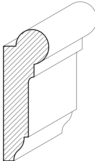
SWPM04 1 \frac{3}{16} " x 2 \frac{3}{8} "
