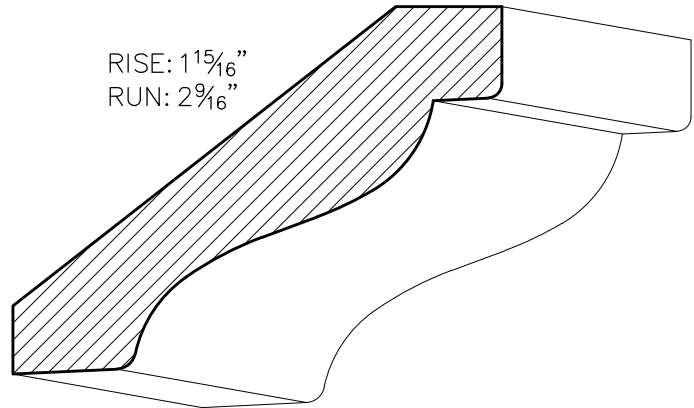
SWCR28 \frac{3}{4}'' \times 3\frac{1}{4}''
