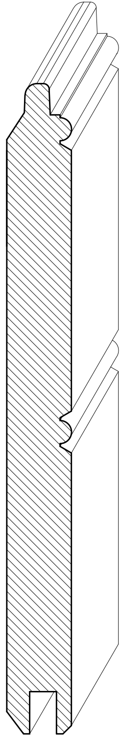
SWPNL12 1\frac{1}{16} " x 6\frac{1}{2} " (Face)
