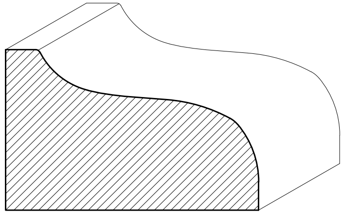
SWOG07 2\frac{1}{16}" \times 1\frac{3}{4}"
