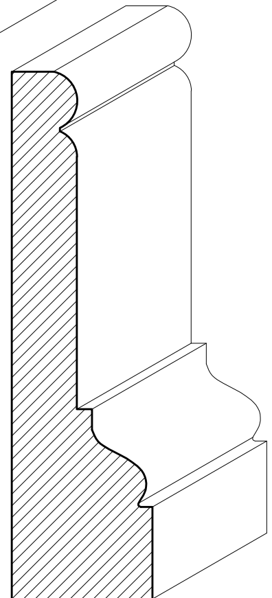
SWCA04 1\frac{1}{6}" \times 4"
