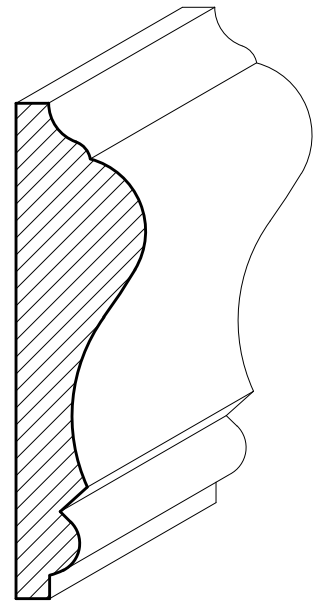
SWCH03 1⅙" x 2½"
