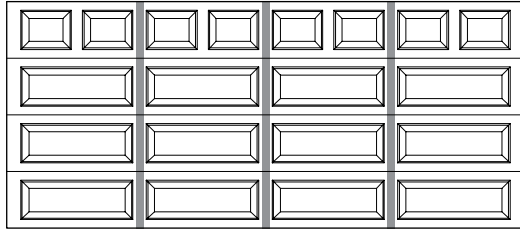
16' wide shown Stile : Centered 1 / Non-centered 2
