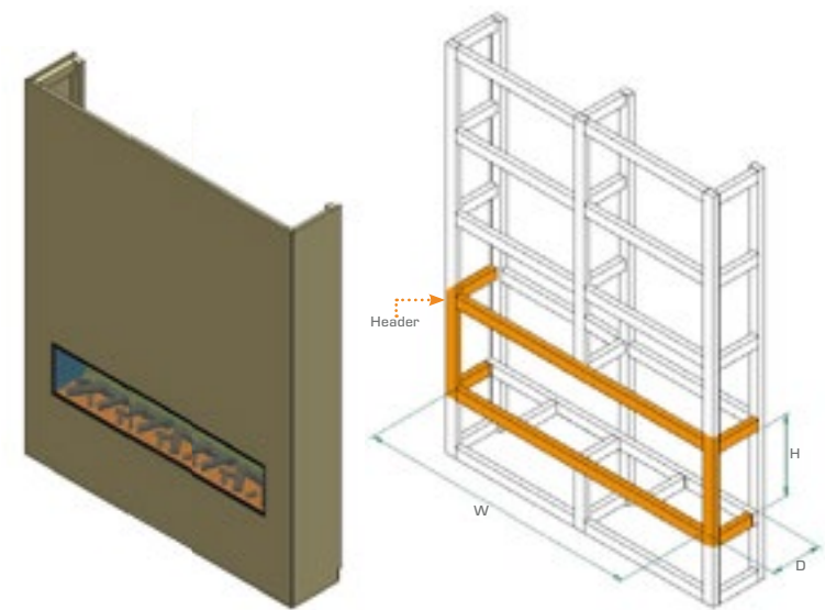
// One-sided (fully-recessed) installation
