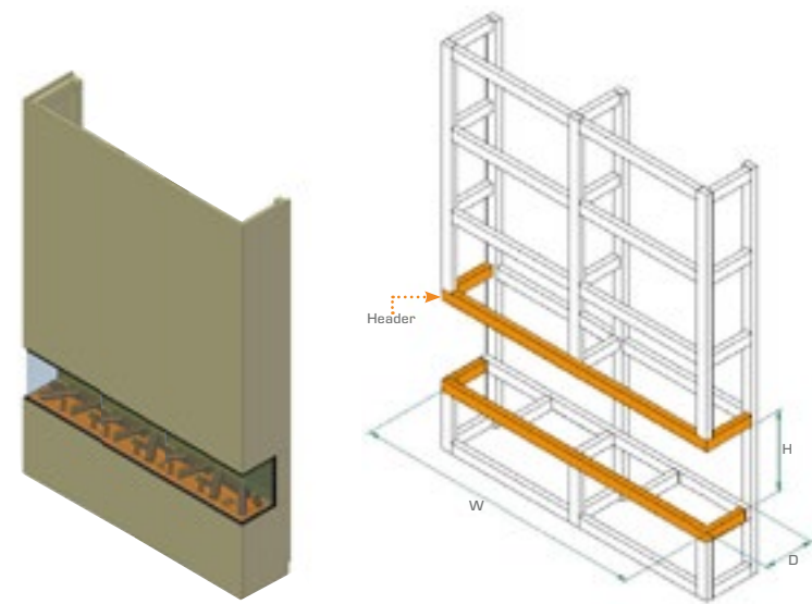
// Three-sided installation
