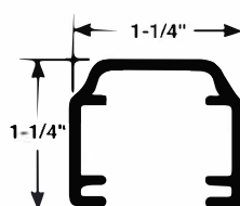
Rail Size
