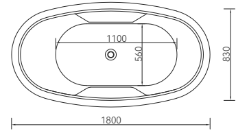
Q435 1800*950*600mm
