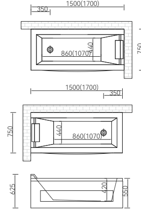
Q351A (L/R) 1500*750*600mm , 1700*750*600mm
