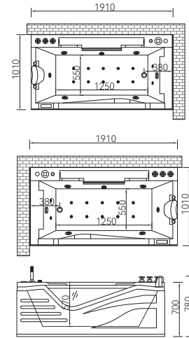
Q325S (L/R) 1910*1010*700mm
