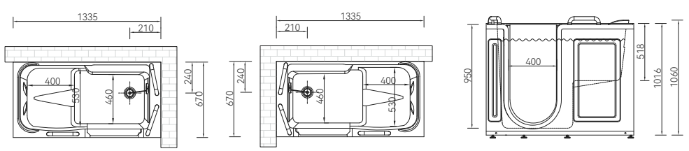
SG5327 (L/R) 1334X673X1060mm
