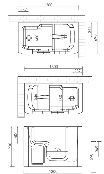
Q372-130 (L/R) 1300*690*900mm
