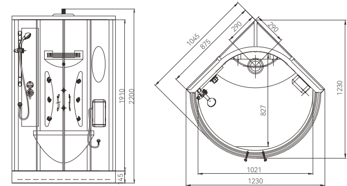
Y811 1045*1045*2200 mm
