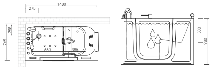
Q377 (L) 1480*765*980mm
