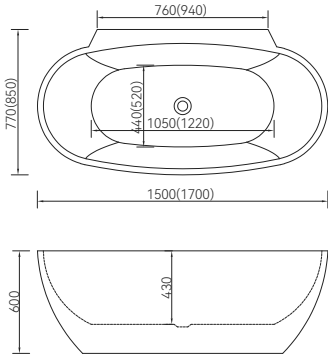
Q360S-170 1700*850*600 mm
