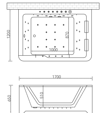
Q450 (L/R) 1700*1200*650mm
