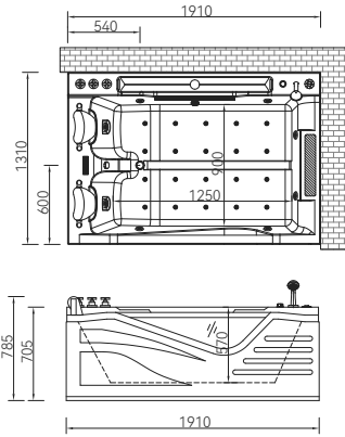
Q325M (R) 1910*1310*705mm
