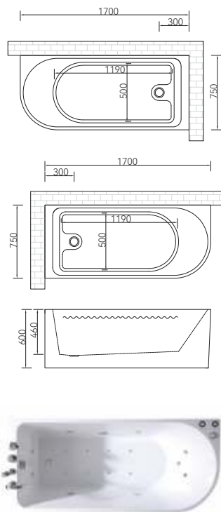
Q368N (L/R) 1700*750*600mm
