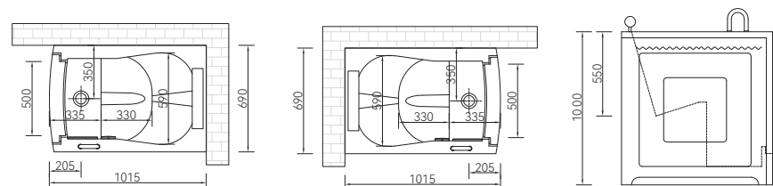
Q376-102 (L/R) 1015*690*1000mm
