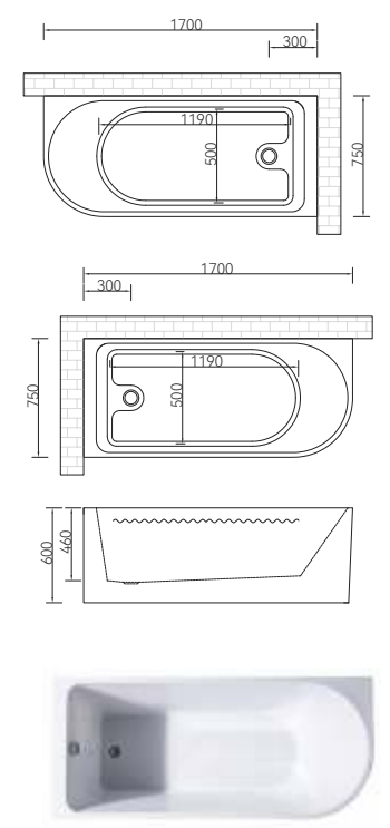
Q368NS (L/R) 1700*750*600mm
