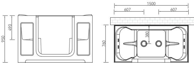
SG5327-150 1500*760*950mm
