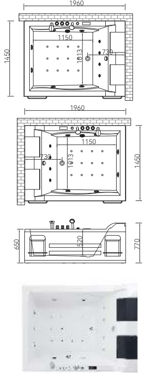
Q410 (L/R) 1960*1450*770mm
