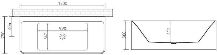
Q410S 1700*750*580mm
