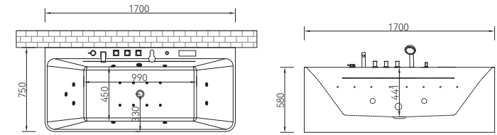
Q410SM 1700*750*580mm
