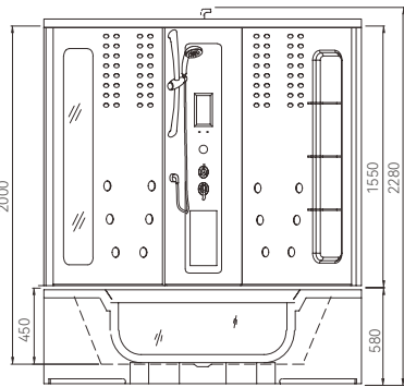
Y842 1510*1510*2280mm
