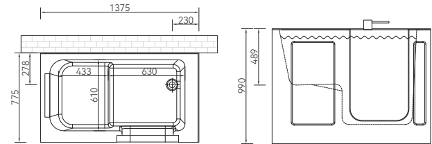
Q378 (R) 1375*775*990mm
