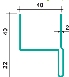
ULS 402 - Kg/mt: 2,94
