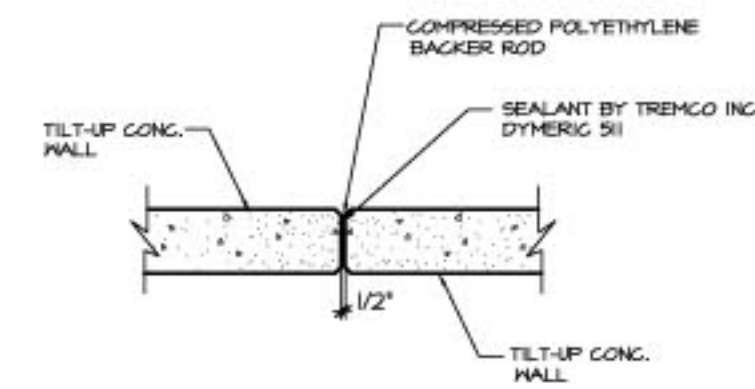
1 JOINT SYSTEM FOR 2HR. WALL U.L. SYSTEM NO. WW-D-0010 SCALE: 1/2" = 1'-0"
