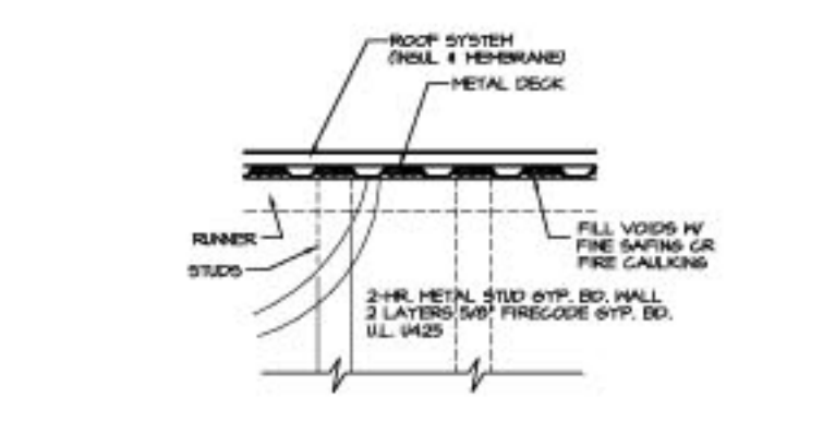
4 2 HR. WALL TERMINATION AT METAL ROOF DECK SCALE: 3/4" = 1'-0"
