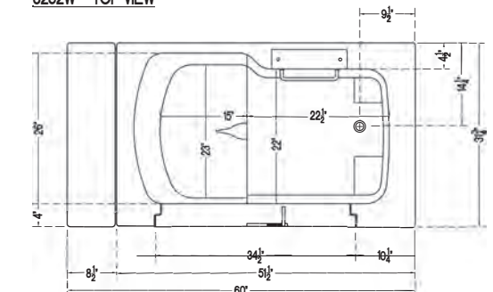
3252W - TOP VIEW
