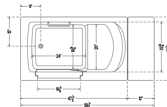
2848 - TOP VIEW
