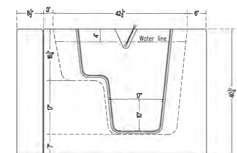
3252W - SIDE VIEW
