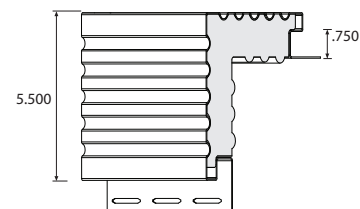
5-1/2" Fluted Outside Corner Post with Foam 20' long 3/4" receiving pocket 6 pieces per carton 120 linear feet per carton
