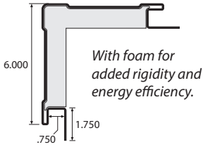
6" Traditional Outside Corner Post with Foam 20' long 3/4" receiving pocket 6 pieces per carton 120 linear feet per carton
