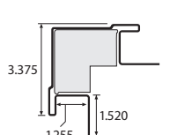
3-1/2" Outside Corner Post with Foam 12' long 1-1/4" receiving pocket 10 pieces per carton 120 linear feet per carton
