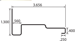
3/4" Window & Door Casing 12' 6" long 20 pieces per carton 250 linear feet per carton
