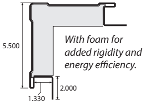
5-1/2" Outside Corner Post with Foam 20' long 1-1/4" receiving pocket 6 pieces per carton 120 linear feet per carton
