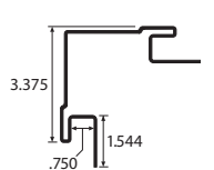
3-1/2" Universal Outside Corner Post 12' long 3/4" receiving pocket 10 pieces per carton 120 linear feet per carton
