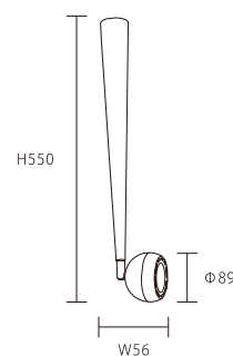
OK 31612 26000 Φ89*W56*H550mm 内附 LED 12W 3000K 鋁材 透鏡玻璃
