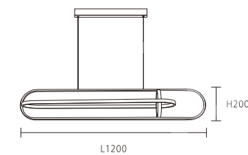
OK 30501 78000 L1200 \times W200 mm 線長:1500mm 內附 LED 45W 3000K 鋼材
