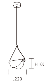
OK 31521 32000 L220*H100mm 線長:1500mm 内含 LED 5W 3000K 鋁材
