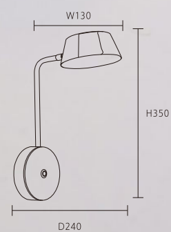
OK 31571 36000 W130*H350*D240mm 內附 LED 8W 3000K 鋼材 附開關
